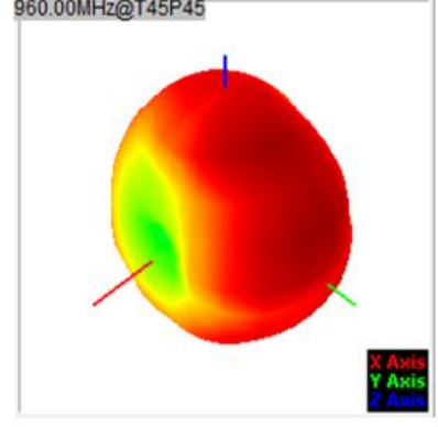
960.00MHz@T45P45
