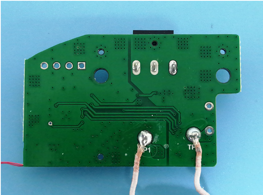
WPT Coil
