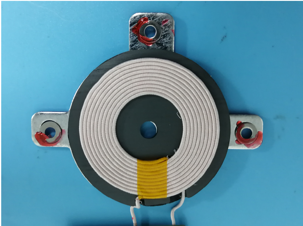
WPT Coil
