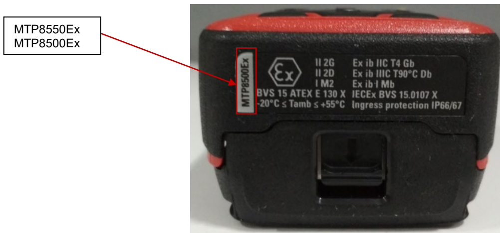
Bottom View with Battery, Model MTP8550Ex / MTP8500Ex
