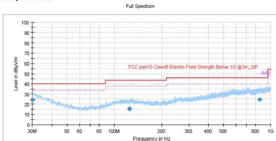
Figure 7: Spectral Diagrams, Radiated Spurious Emission, 30MHz-1000MHz, Horizontal, mode A.3
