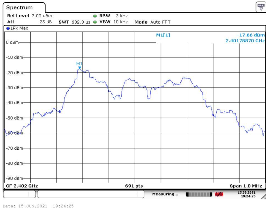
Figure 3: Power Spectral Density Measurement
