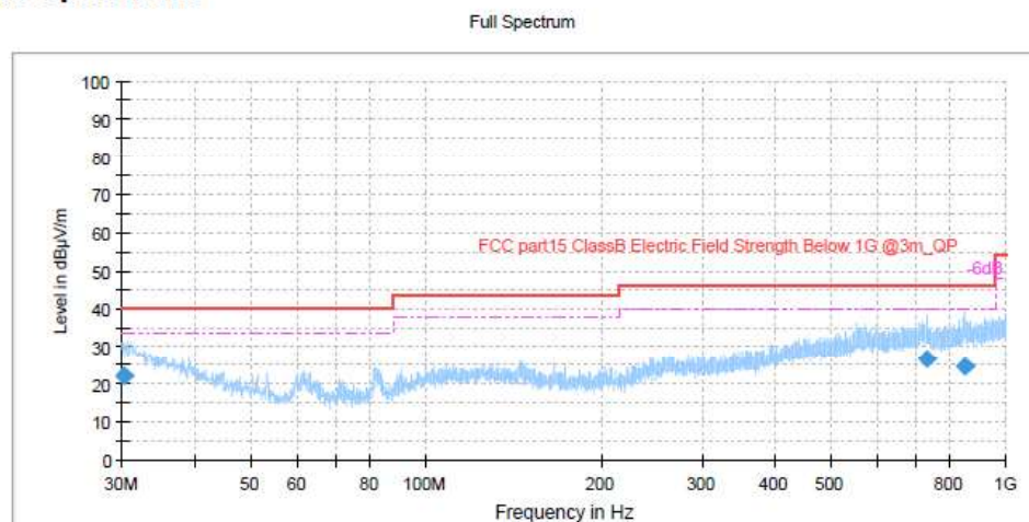
Figure 10: Spectral Diagrams, Radiated Spurious Emission, 30MHz-1000MHz, Vertical, mode B.1
