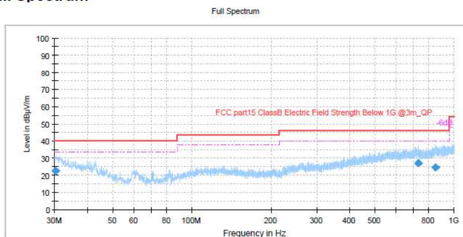
Figure 8: Spectral Diagrams, Radiated Spurious Emission, 30MHz-1000MHz, Vertical, mode A.3
