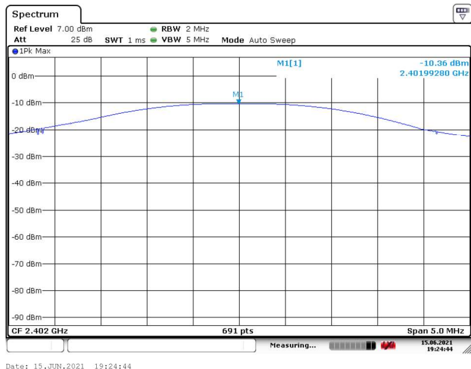
Figure 2: Maximum peak Conducted Output Power Measurement
