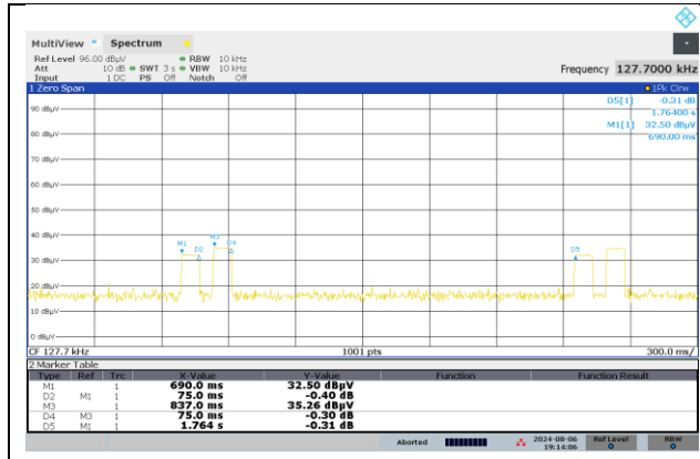
CONFIGURATION 1 (127.7kHz)
