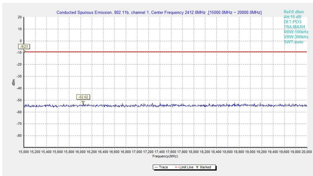
Fig.A.6.1.7 Conducted Spurious Emission (802.11b, Ch1, 15 GHz-20 GHz)
