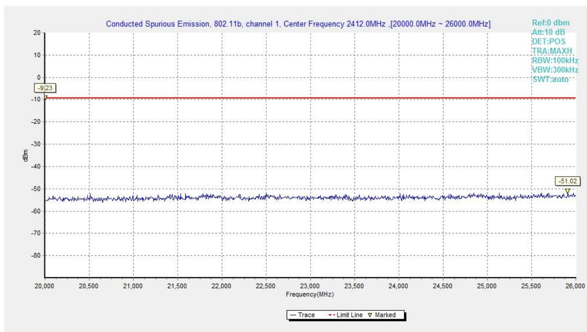
Fig.A.6.1.8 Conducted Spurious Emission (802.11b, Ch1, 20 GHz-26 GHz)
