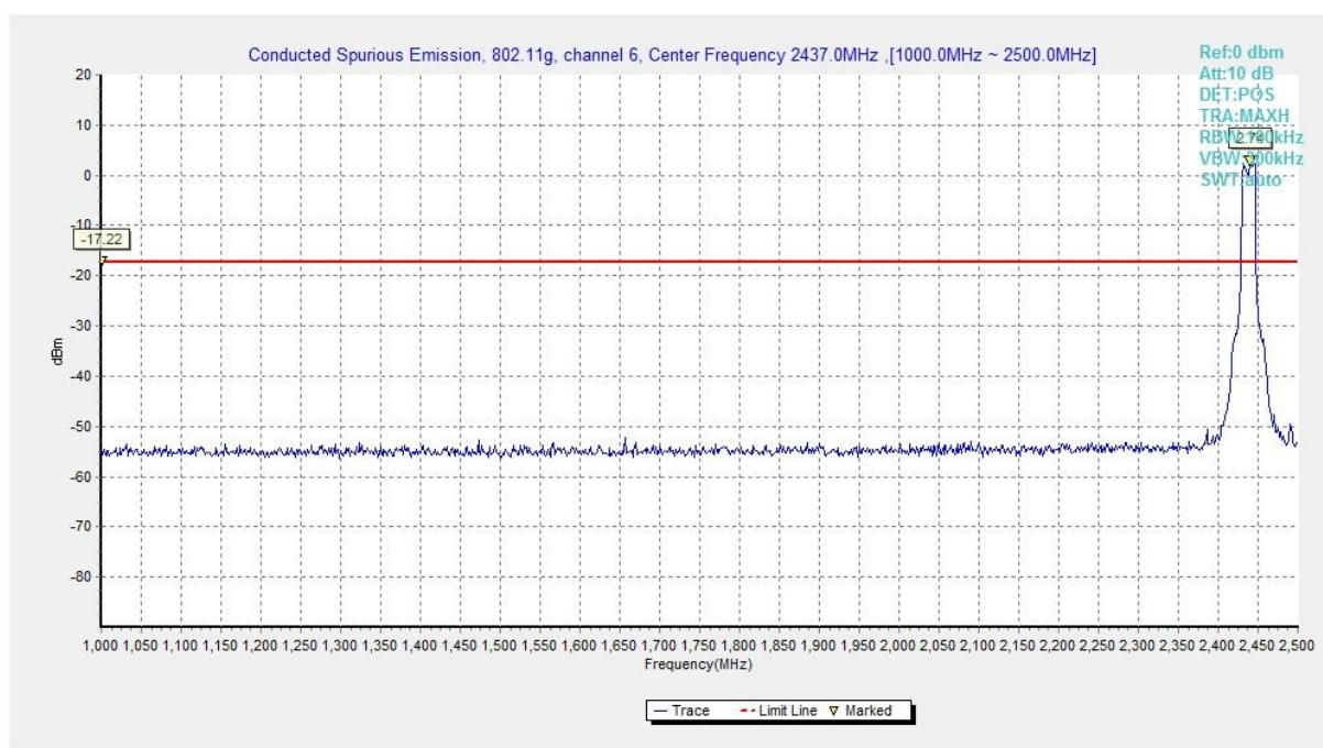
Fig.A.6.1.35 Conducted Spurious Emission (802.11g, Ch6, 1 GHz-2.5 GHz)
