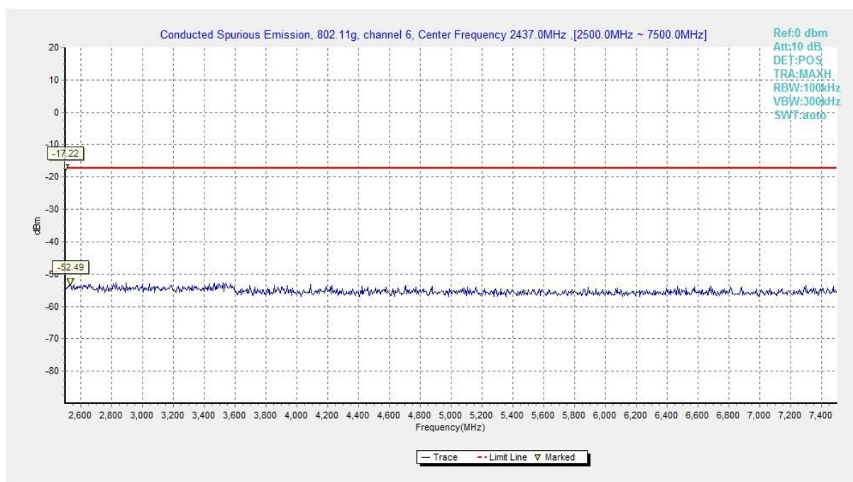
Fig.A.6.1.36 Conducted Spurious Emission (802.11g, Ch6, 2.5 GHz-7.5 GHz)
