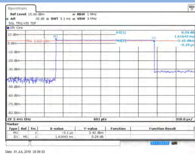
GFSK DH3
