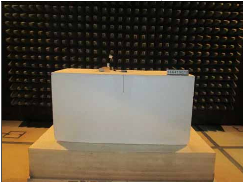
Radiated Emission Test above 1GHz (Part 15.247)
