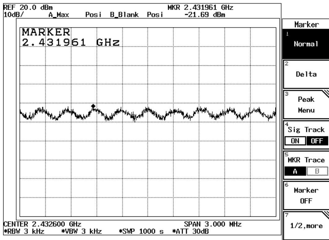
Figure Channel 6: 54Mbps
