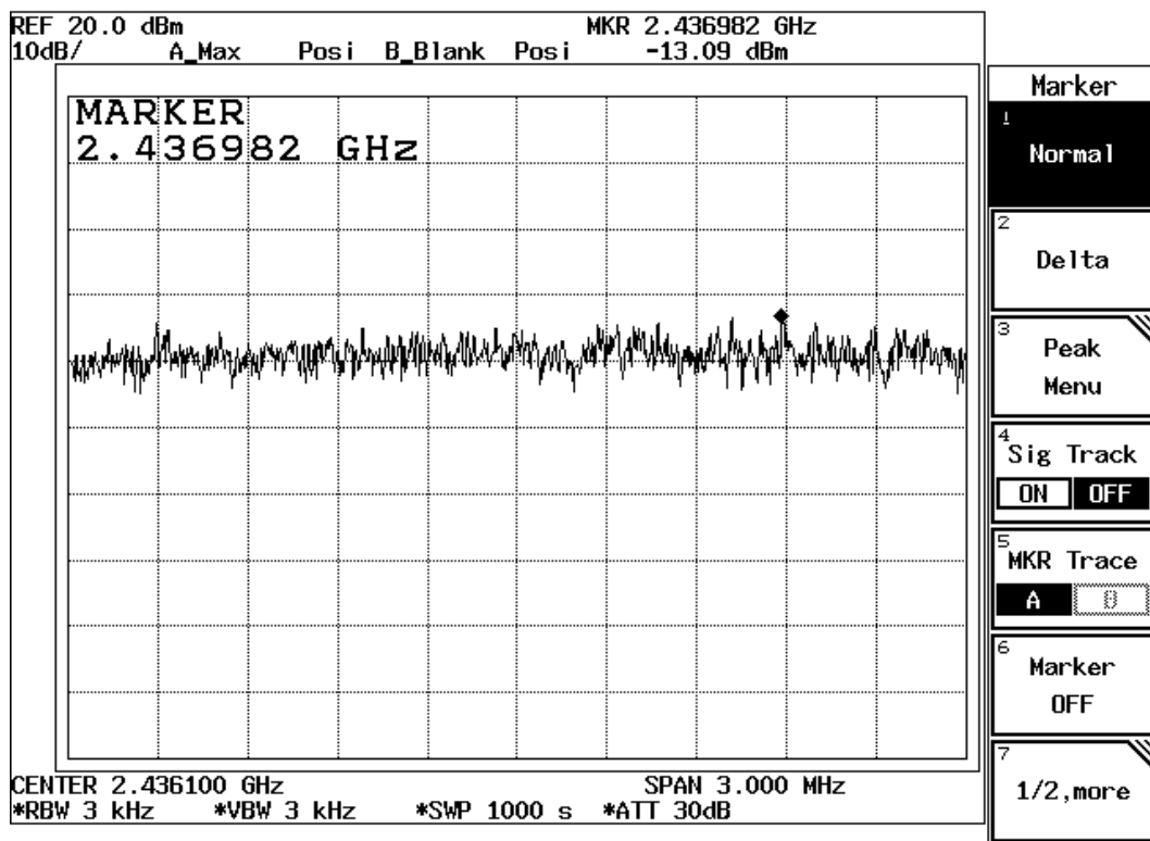
Figure Channel 6: 11Mbps
