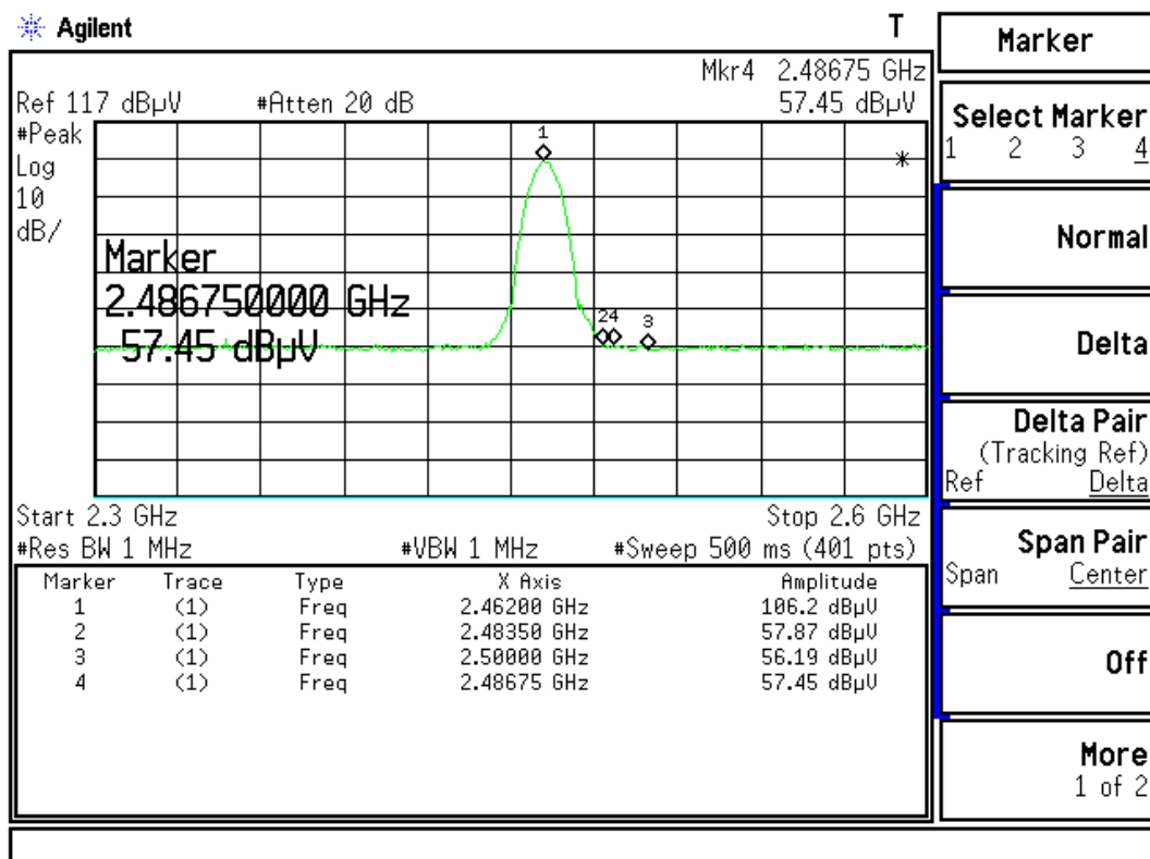
Figure Channel 11: (Vertical)
