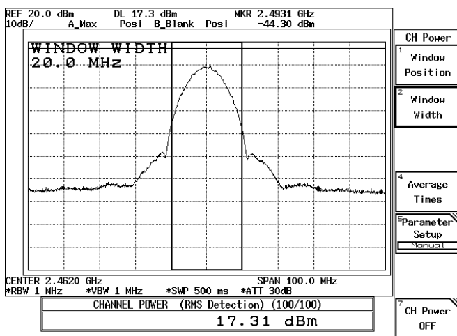
11Mbps-CH11
