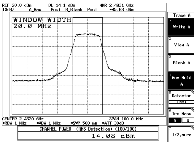
54Mbps-CH11
