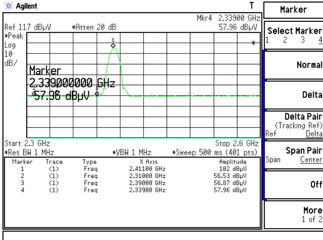
Figure Channel 1: (Horizontal)
