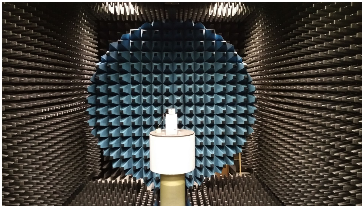
Figure 1: Antenna chamber
