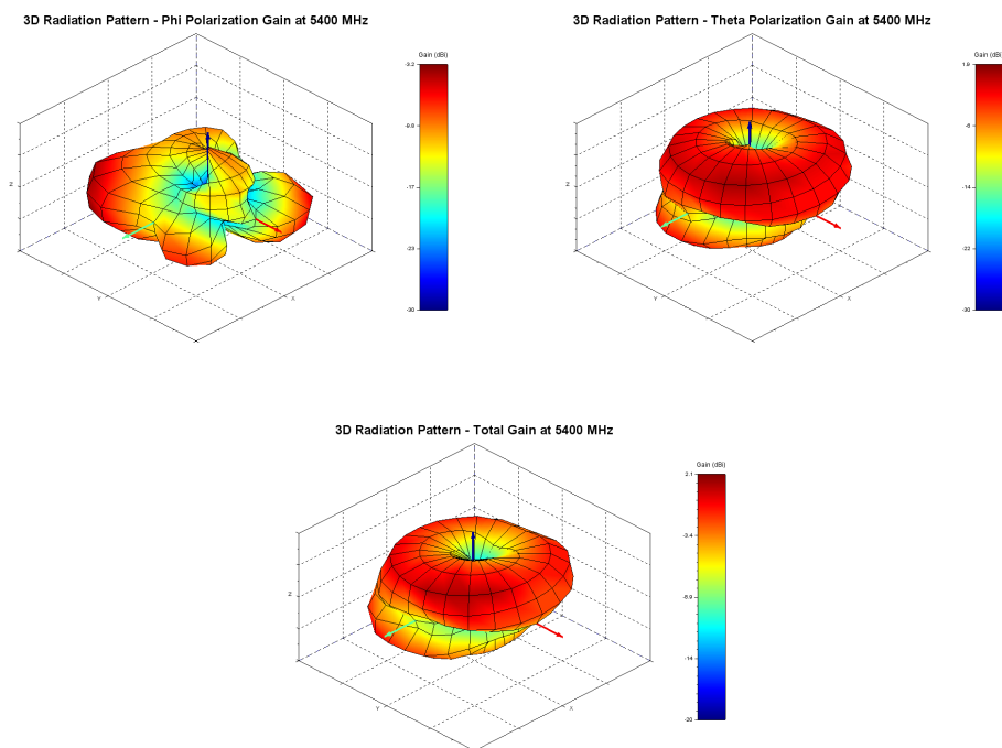
Figure 9: Phi, Theta, and total gain plots
