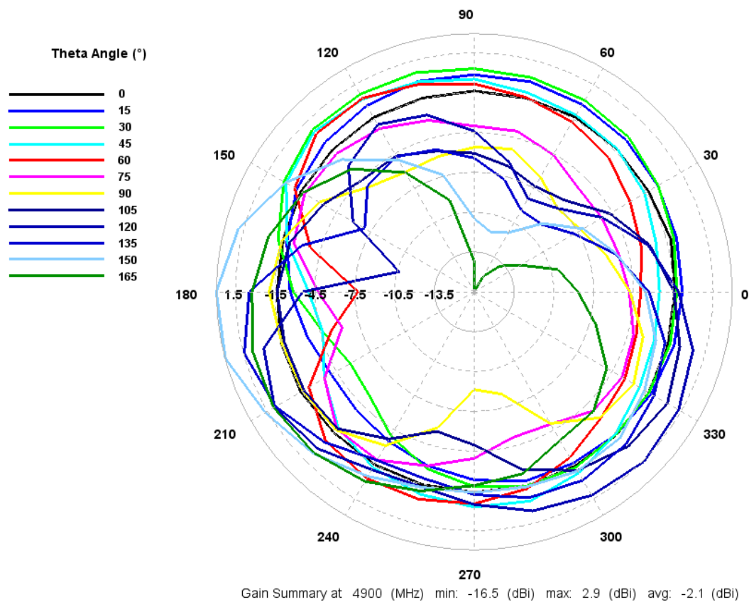
Figure 15: Total gain pattern
