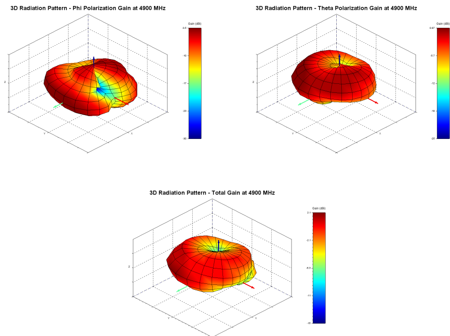
Figure 7: Phi, Theta, and total gain plots
