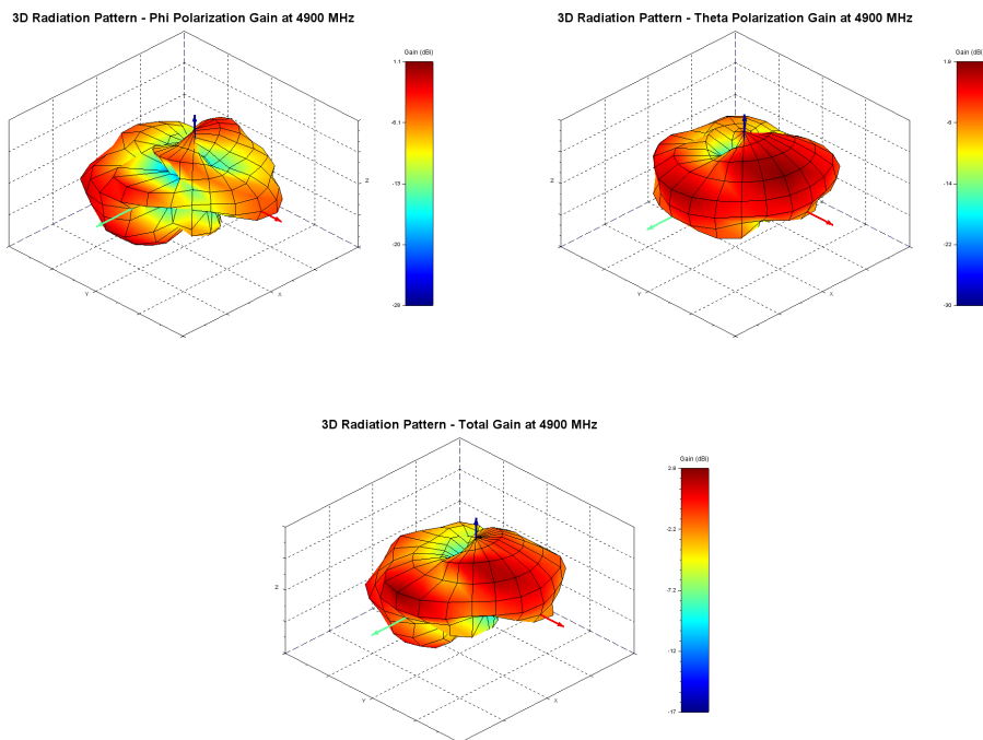
Figure 25: Phi, Theta, and total gain plots
