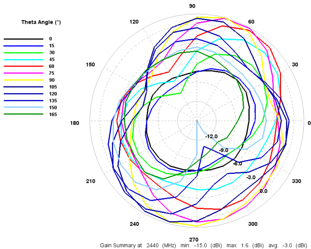
Figure 22: Total gain pattern
