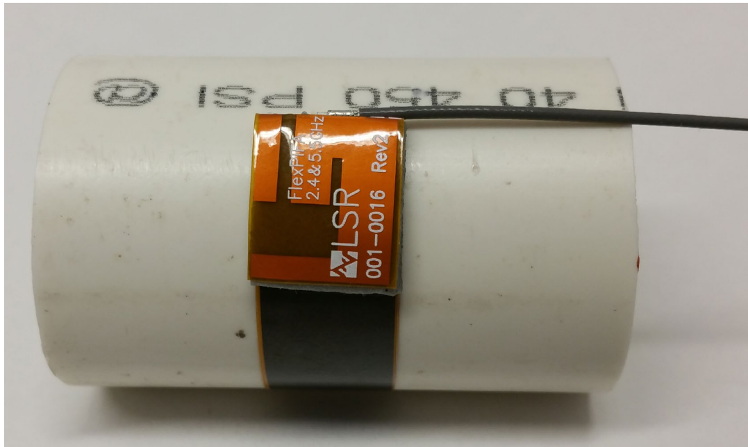
Figure 34: Convex-mounted
