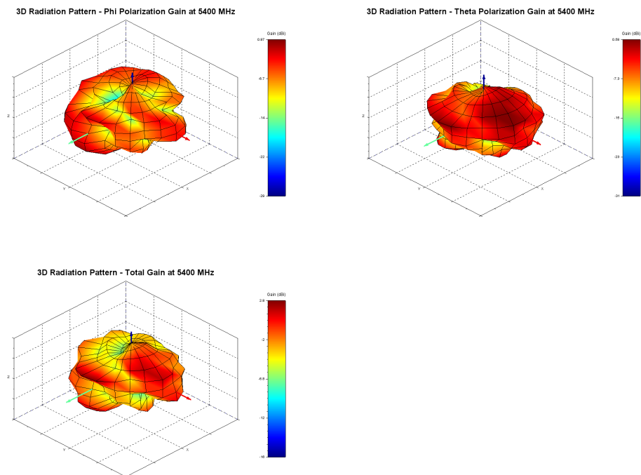
Figure 27: Phi, Theta, and total gain plots
