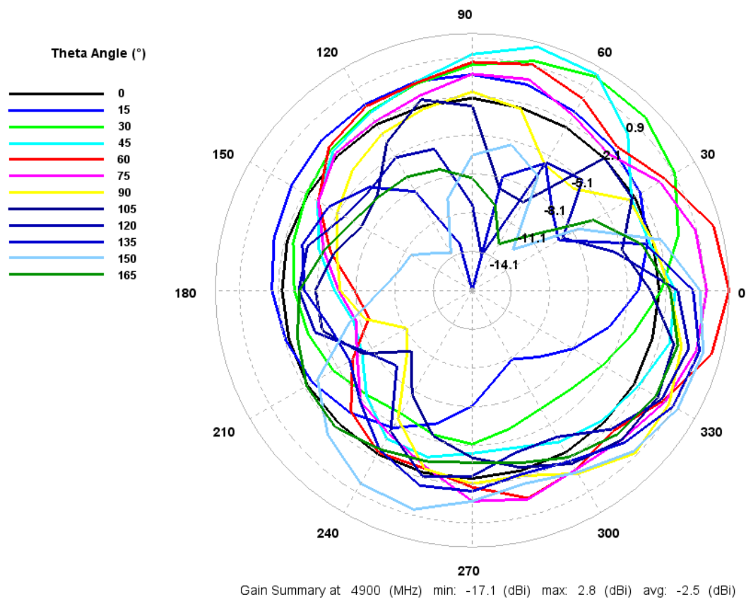
Figure 24: Total gain pattern
