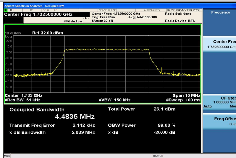
Band4-5MHz-16QAM-20175-25RB#0-4.4835
