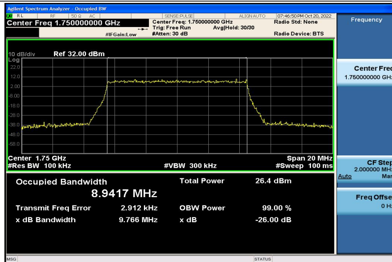
Band4-10MHz-16QAM-20350-50RB#0-8.9417
