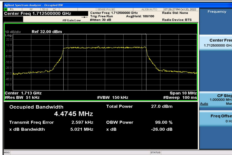
Band4-5MHz-QPSK-19975-25RB#0-4.4745
