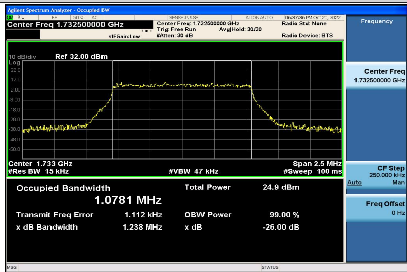
Band4-1.4MHz-16QAM-20175-6RB#0-1.0781
