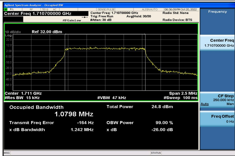
Band4-1.4MHz-16QAM-19957-6RB#0-1.0798
