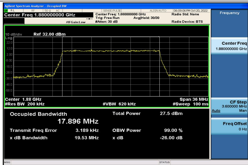
Band2-20MHz-16QAM-18900-100RB#0-17.896
