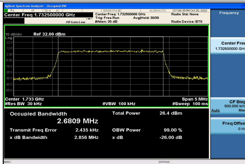
Band4-3MHz-QPSK-20175-15RB#0-2.6809
