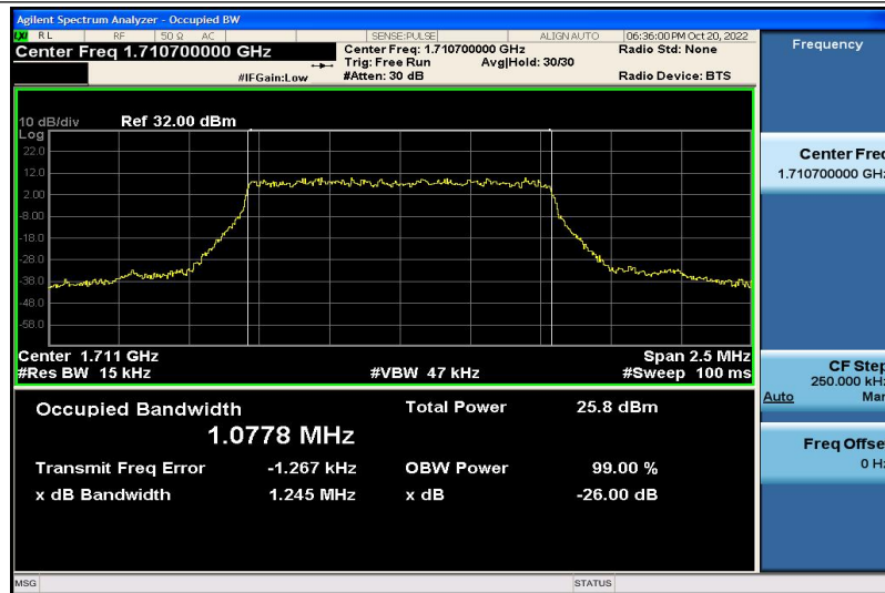
Band4-1.4MHz-QPSK-19957-6RB#0-1.0778
