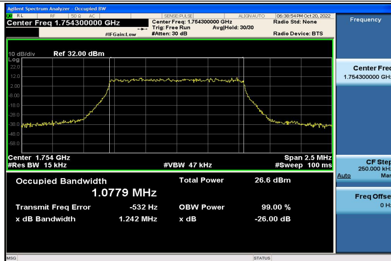
Band4-1.4MHz-QPSK-20393-6RB#0-1.0779
