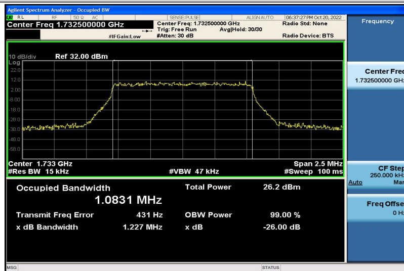
Band4-1.4MHz-QPSK-20175-6RB#0-1.0831
