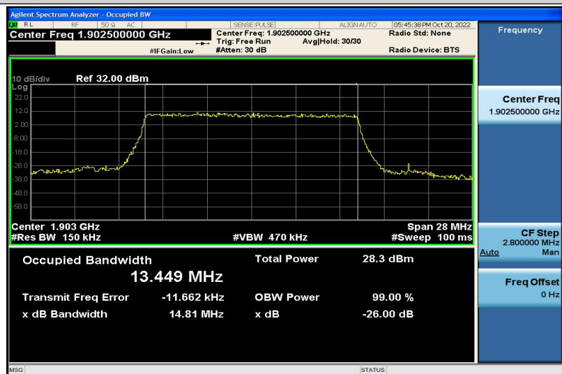
Band2-15MHz-QPSK-19125-75RB#0-13.449
