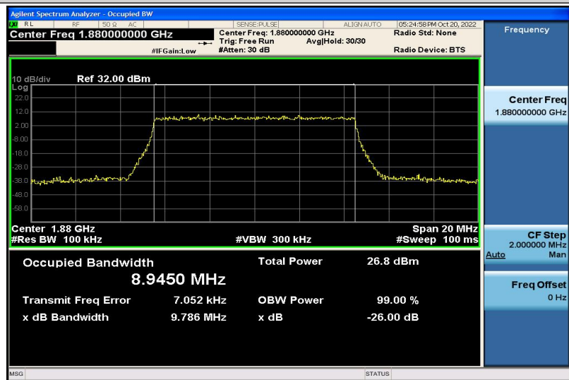
Band2-10MHz-16QAM-18900-50RB#0-8.9450
