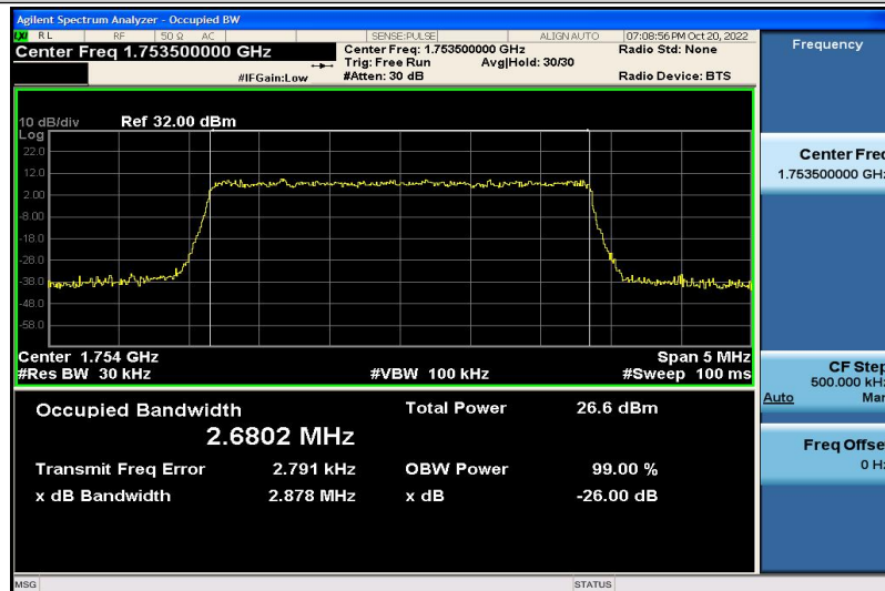
Band4-3MHz-QPSK-20385-15RB#0-2.6802
