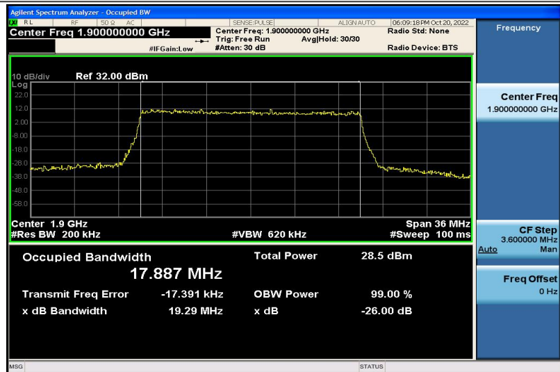
Band2-20MHz-QPSK-19100-100RB#0-17.887
