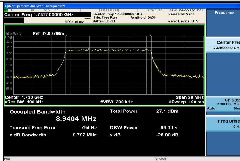
Band4-10MHz-QPSK-20175-50RB#0-8.9404
