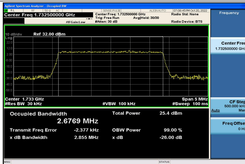
Band4-3MHz-16QAM-20175-15RB#0-2.6769
