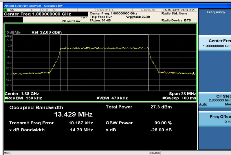
Band2-15MHz-16QAM-18900-75RB#0-13.429
