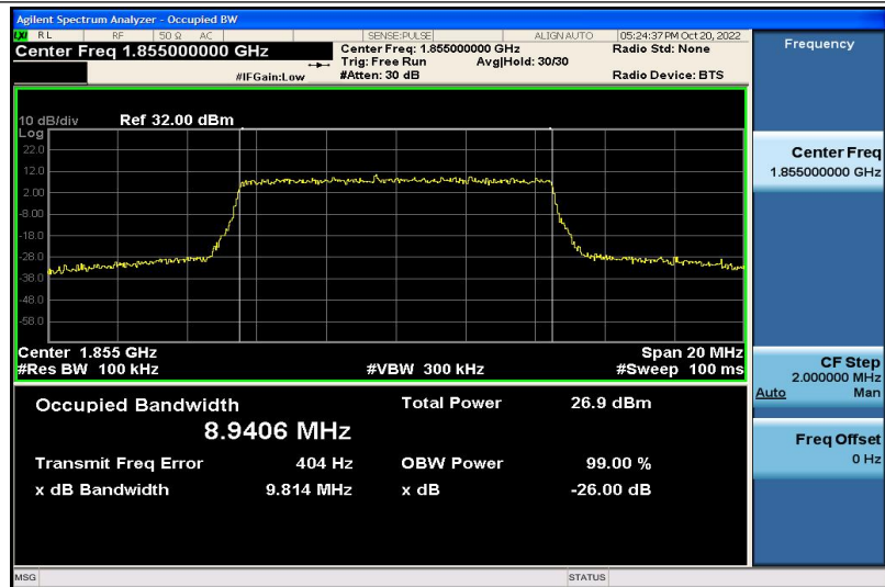
Band2-10MHz-16QAM-18650-50RB#0-8.9406
