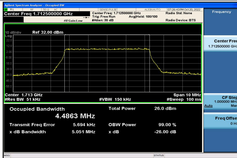
Band4-5MHz-16QAM-19975-25RB#0-4.4863
