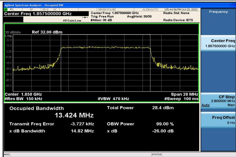
Band2-15MHz-QPSK-18675-75RB#0-13.424
