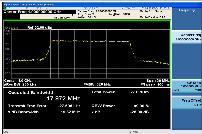
Band2-20MHz-16QAM-19100-100RB#0-17.872
