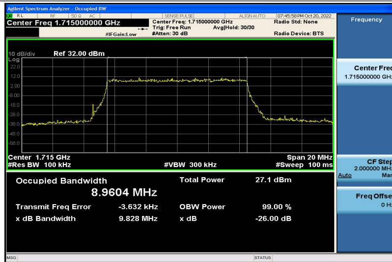
Band4-10MHz-QPSK-20000-50RB#0-8.9604
