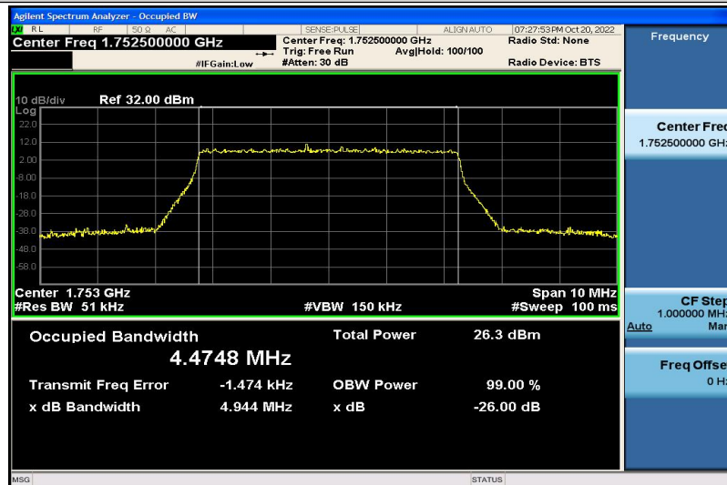
Band4-5MHz-16QAM-20375-25RB#0-4.4748
