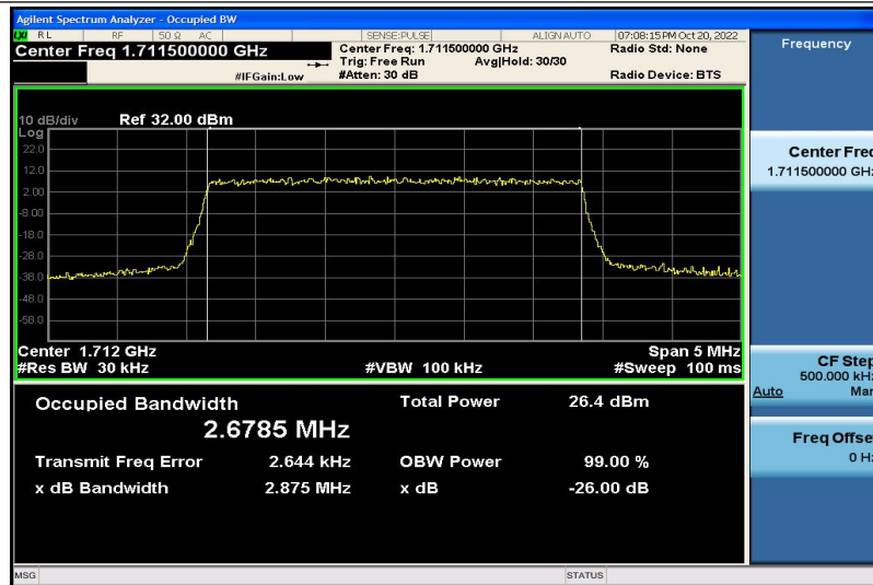
Band4-3MHz-QPSK-19965-15RB#0-2.6785
