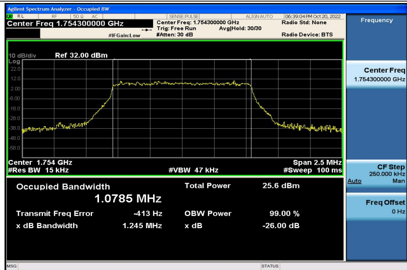
Band4-1.4MHz-16QAM-20393-6RB#0-1.0785
