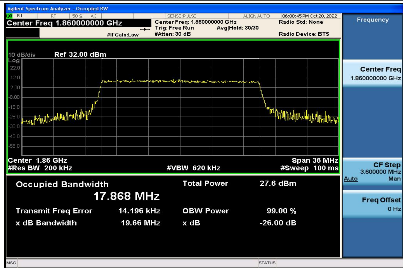
Band2-20MHz-16QAM-18700-100RB#0-17.868
