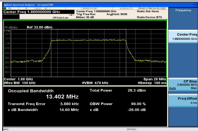
Band2-15MHz-QPSK-18900-75RB#0-13.402
