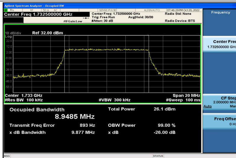
Band4-10MHz-16QAM-20175-50RB#0-8.9485
