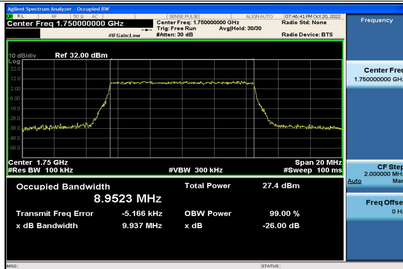
Band4-10MHz-QPSK-20350-50RB#0-8.9523
