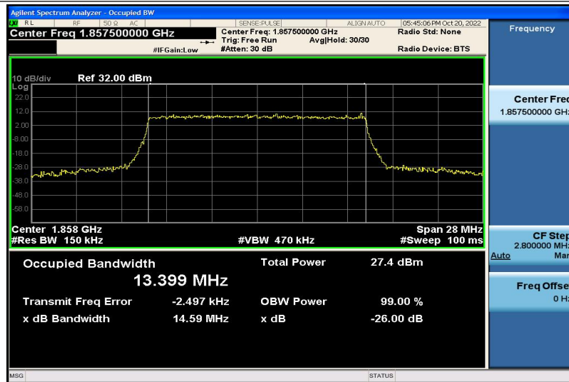
Band2-15MHz-16QAM-18675-75RB#0-13.399
