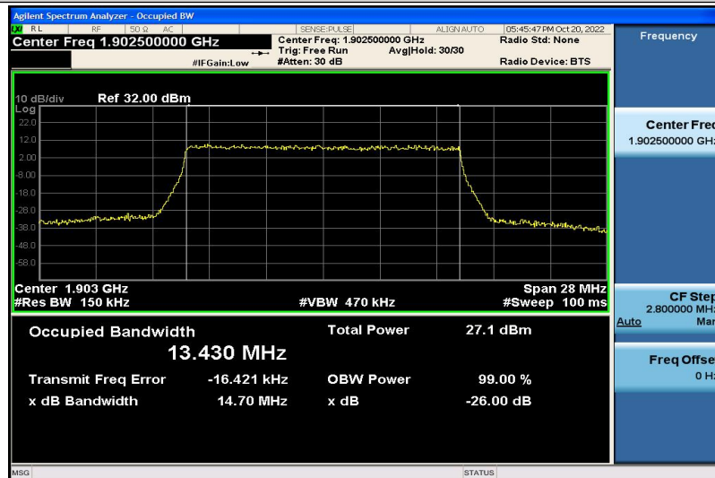
Band2-15MHz-16QAM-19125-75RB#0-13.430
