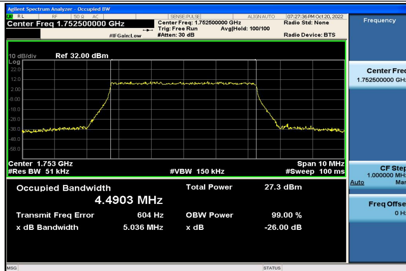
Band4-5MHz-QPSK-20375-25RB#0-4.4903
