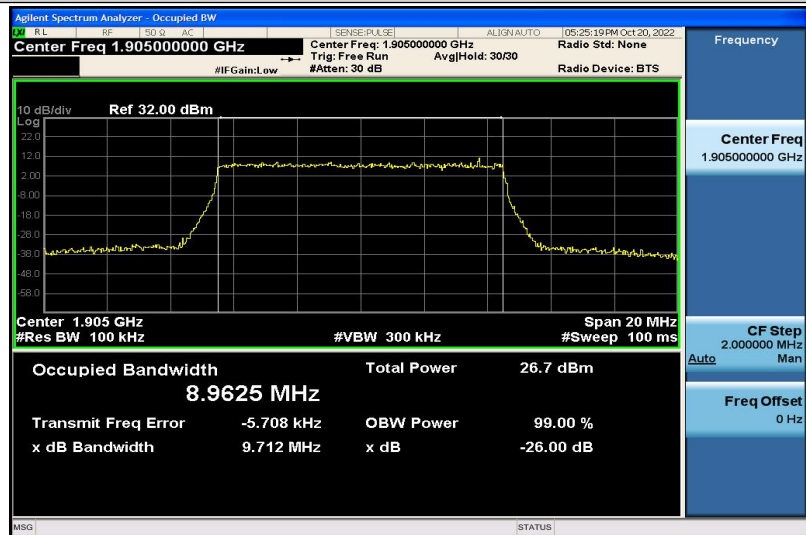
Band2-10MHz-16QAM-19150-50RB#0-8.9625
