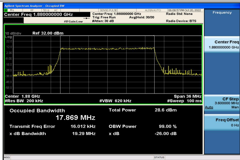
Band2-20MHz-QPSK-18900-100RB#0-17.869
