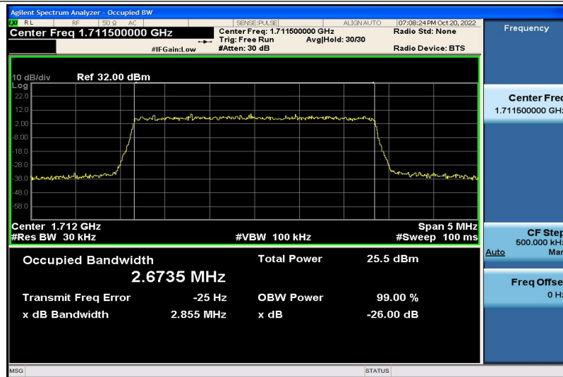
Band4-3MHz-16QAM-19965-15RB#0-2.6735
