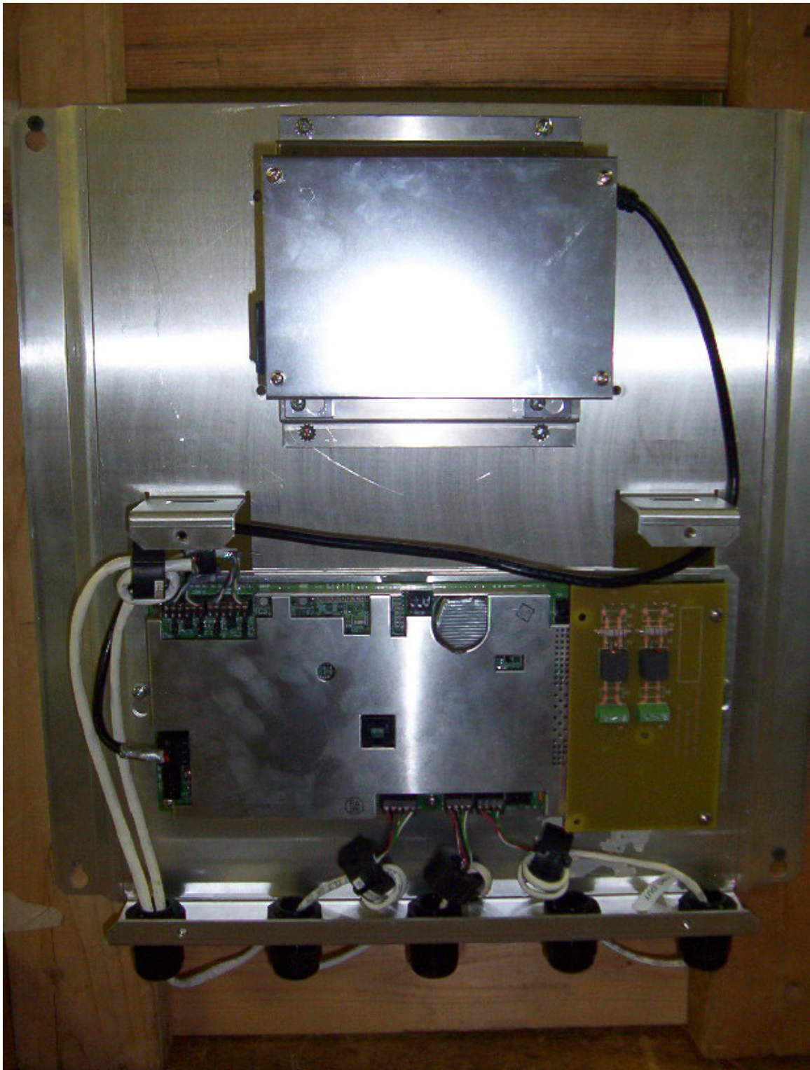
Liberty FX Power Supply & TR4024 Controller cover removed
