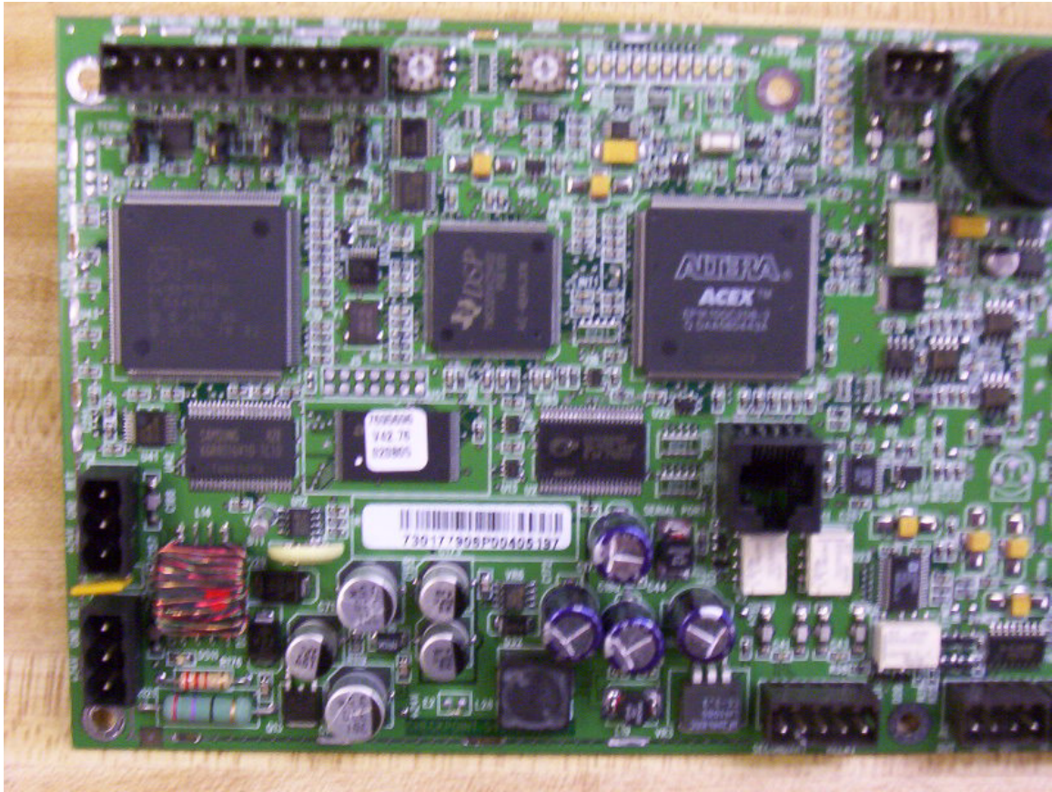
Liberty FX TR4024 PCB Component Right Side
