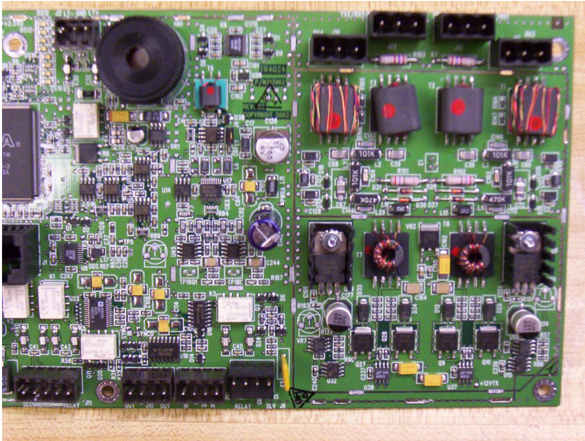
Liberty FX TR4024 PCB Component Left Side
