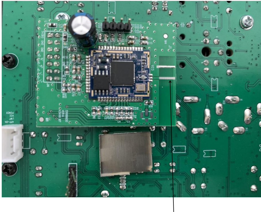
PCB antenna
