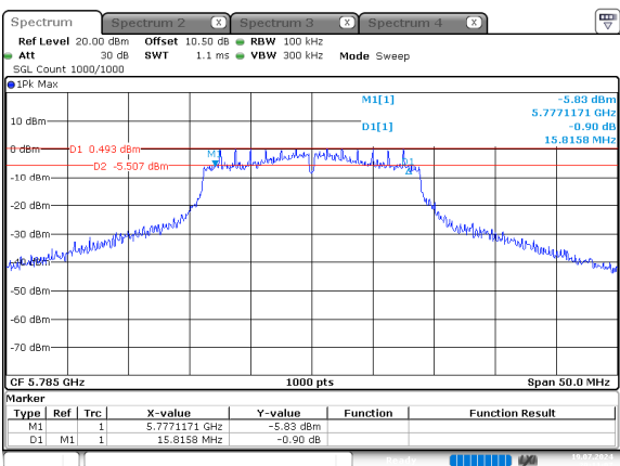
n20_5785MHz_Chain 0
