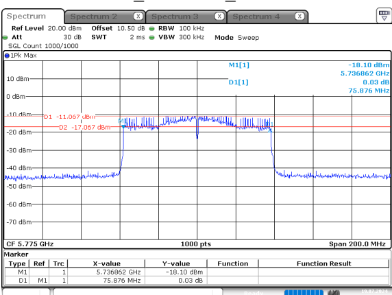
ac80_5775MHz_Chain 0
