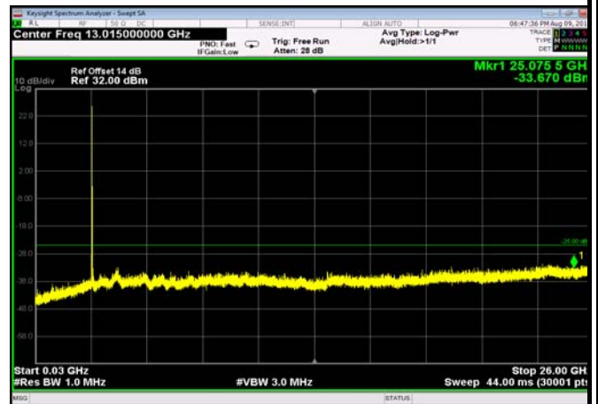
TDD41_HighRange_5MHz_30MHz~26GHz
