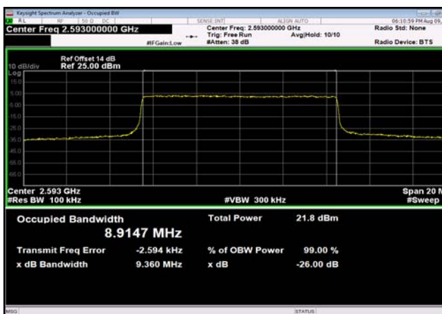
TDD41_MidRange_15_2593_QPSK
