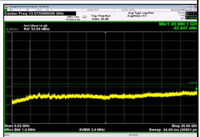
TDD41_MidRange_15MHz_30MHz~26GHz
