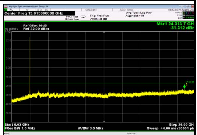
TDD41_MidRange_5MHz_30MHz~26GHz
