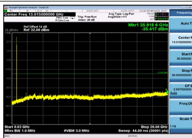
FDD05_MidRange_3MHz_30MHz~26GHz
