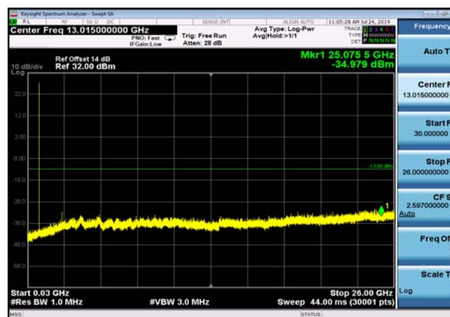
FDD05_LowRange_1.4MHz_30MHz~26GHz
