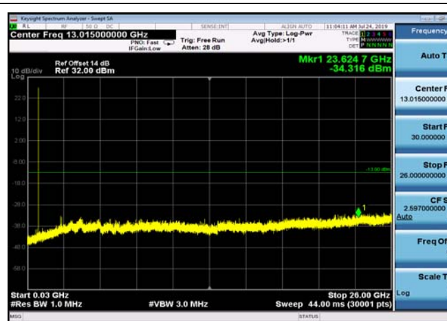
FDD05_MidRange_1.4MHz_30MHz~26GHz
