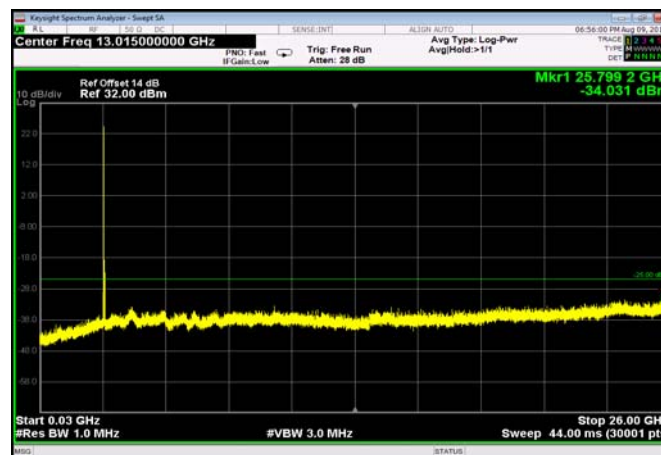
TDD41_LowRange_10MHz_30MHz~26GHz
