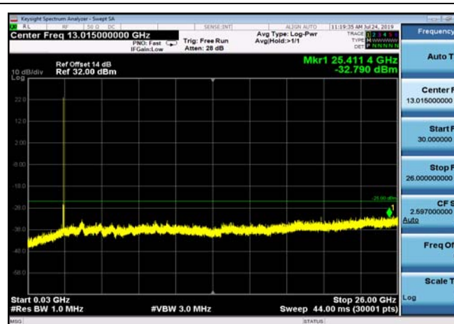
FDD07_MidRange_20MHz_30MHz~26GHz
