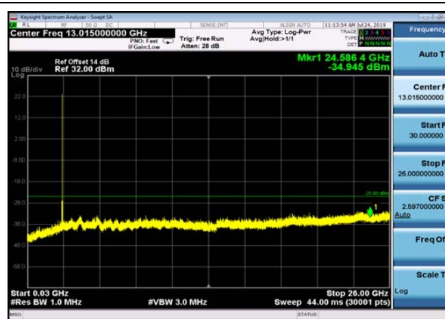
FDD07_MidRange_20MHz_30MHz~26GHz
