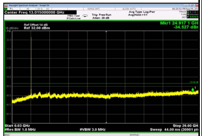
TDD41_LowRange_15MHz_30MHz~26GHz
