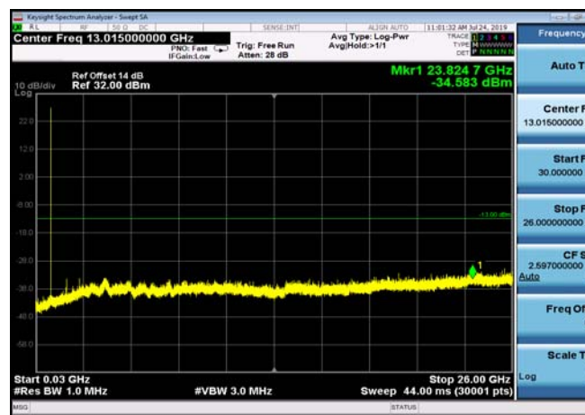
FDD05_HighRange_3MHz_30MHz~26GHz
