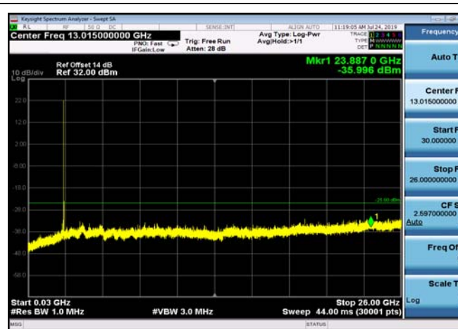
FDD07_MidRange_10MHz_30MHz~26GHz
