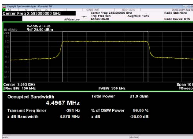
TDD41_MidRange_5MHz_2593MHz_QPSK
