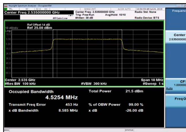
FDD07_MidRange_10_2535_QPSK
