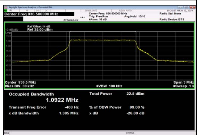
FDD05_MidRange_3_836.5_Q16
