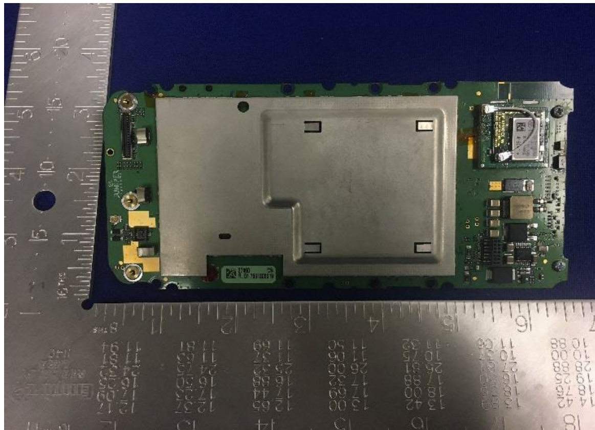
Main Board - Back
