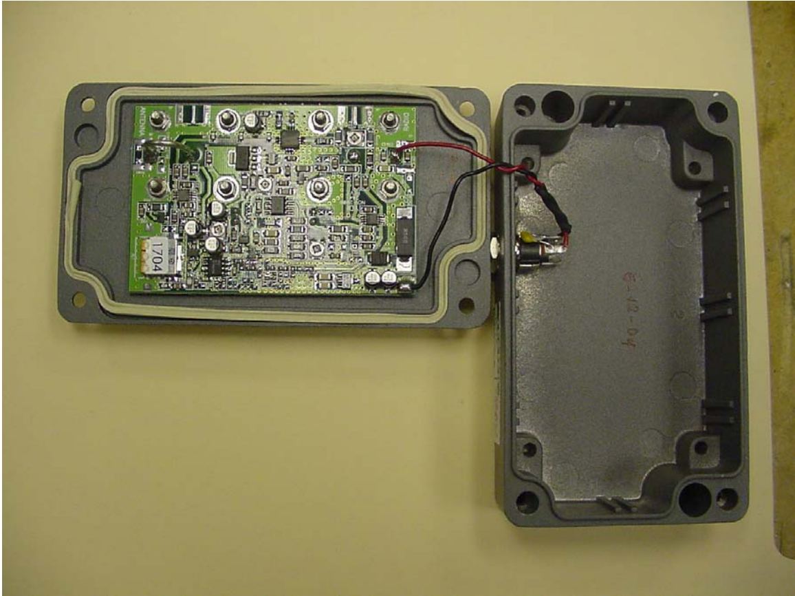
Interior of device enclosure with cover removed.
