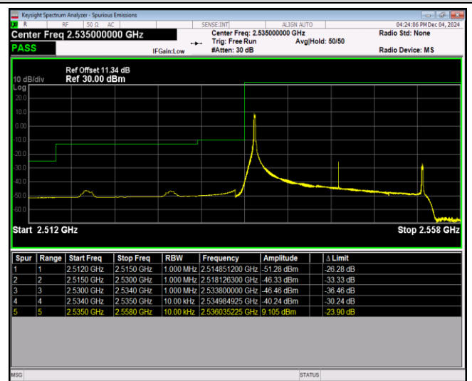
Band41-20MHz-16QAM-40140-100RB#0
