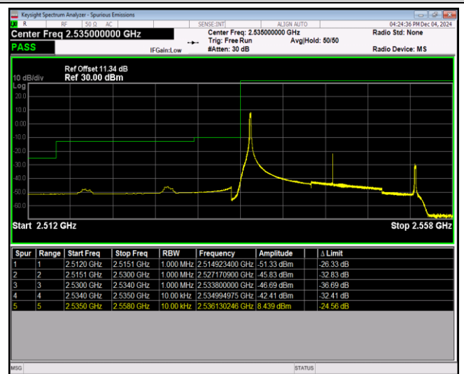
Band41-20MHz-64QAM-40140-100RB#0
