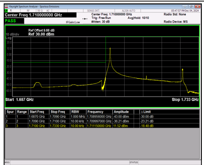
Band66-20MHz-16QAM-132072-100RB#0
