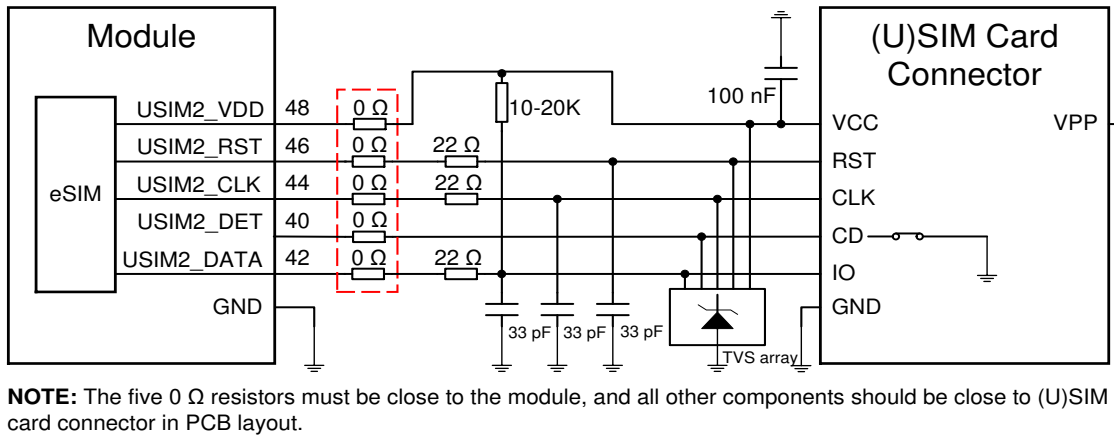
Figure 16: Recommended Compatible Design for (U)SIM2 Interface
