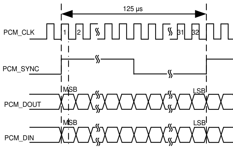
Figure 19: Auxiliary Mode Timing
