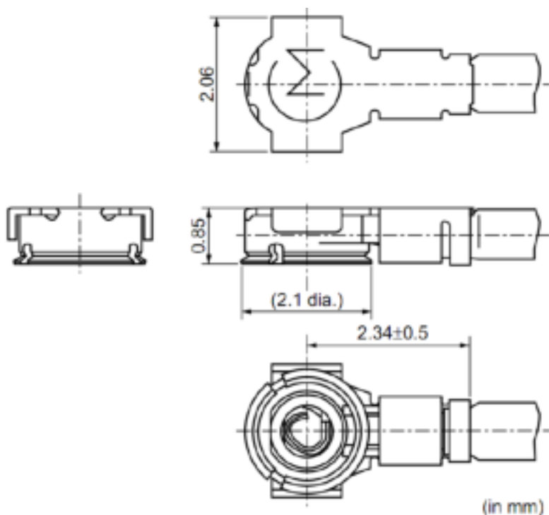
Figure 26: Dimensions of Mated Plugs ( \varnothing 0.81/ \varnothing 1.13 mm Coaxial Cables) (Unit: mm)
