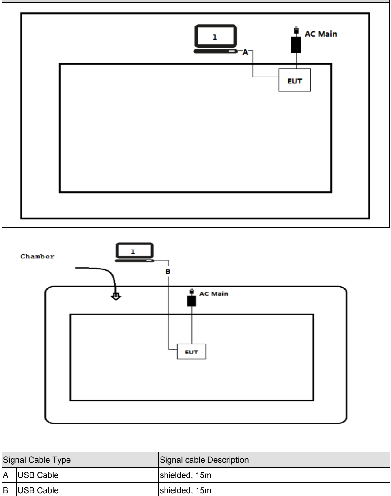
Connection Diagram
