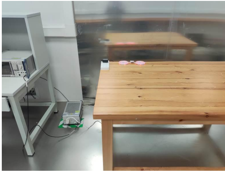
radiation L
