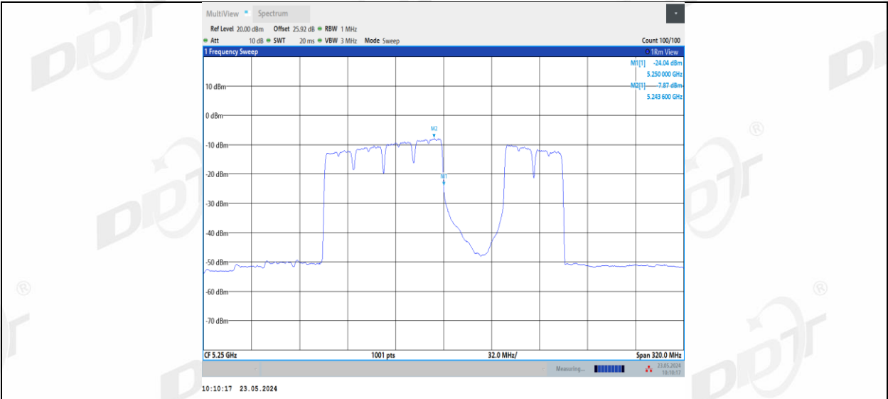
11BE160MIMO Ant2 5250 UNII-1 996+484 Non-OFDMA 4
