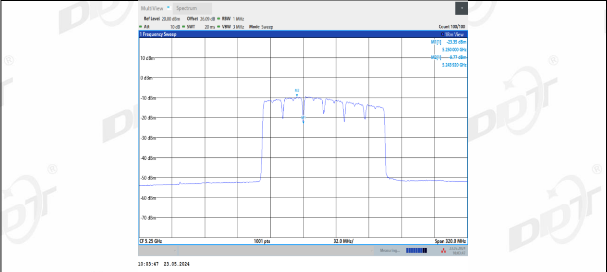
11BE160MIMO Ant3 5250 UNII-1 996+484 Non-OFDMA 2
