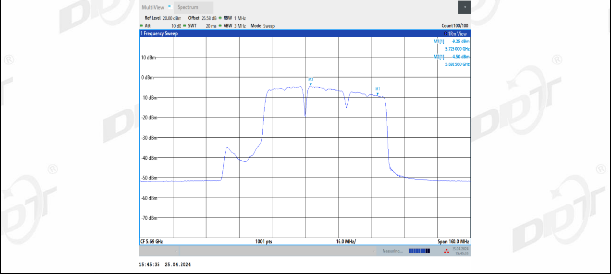
11BE80MIMO Ant3 5690 UNII-2C 484+242 Non-OFDMA 2
