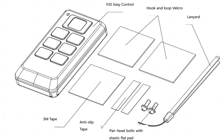
Figure 2 Components of FJD Easy Control
