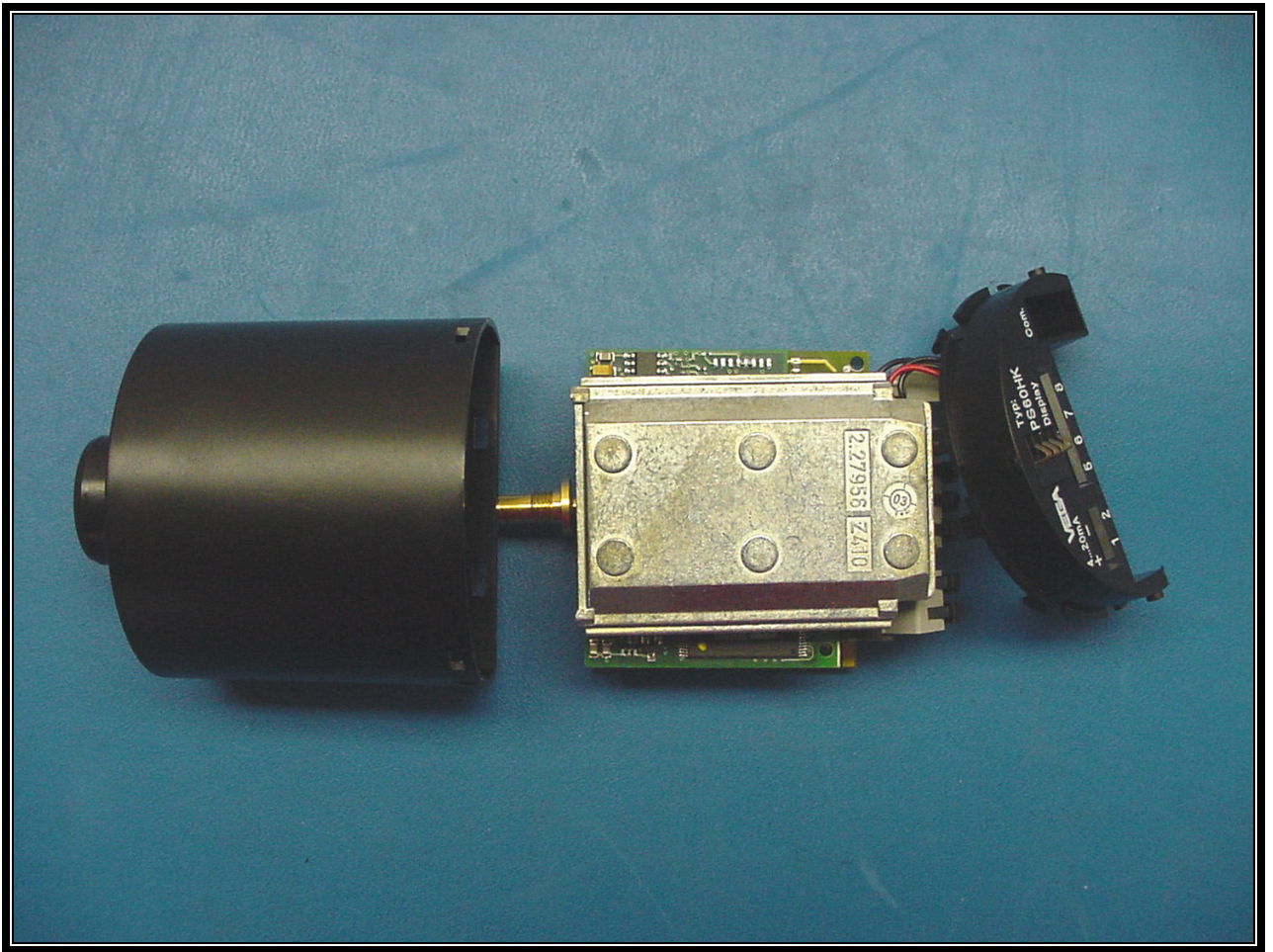
PHOTOGRAPH 27: EUT MODULE PARTS INSIDE VIEW
