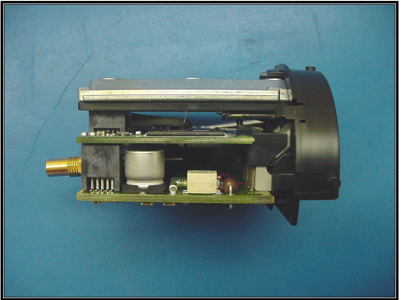
PHOTOGRAPH 28: EUT MODULE PARTS SIDE VIEW
