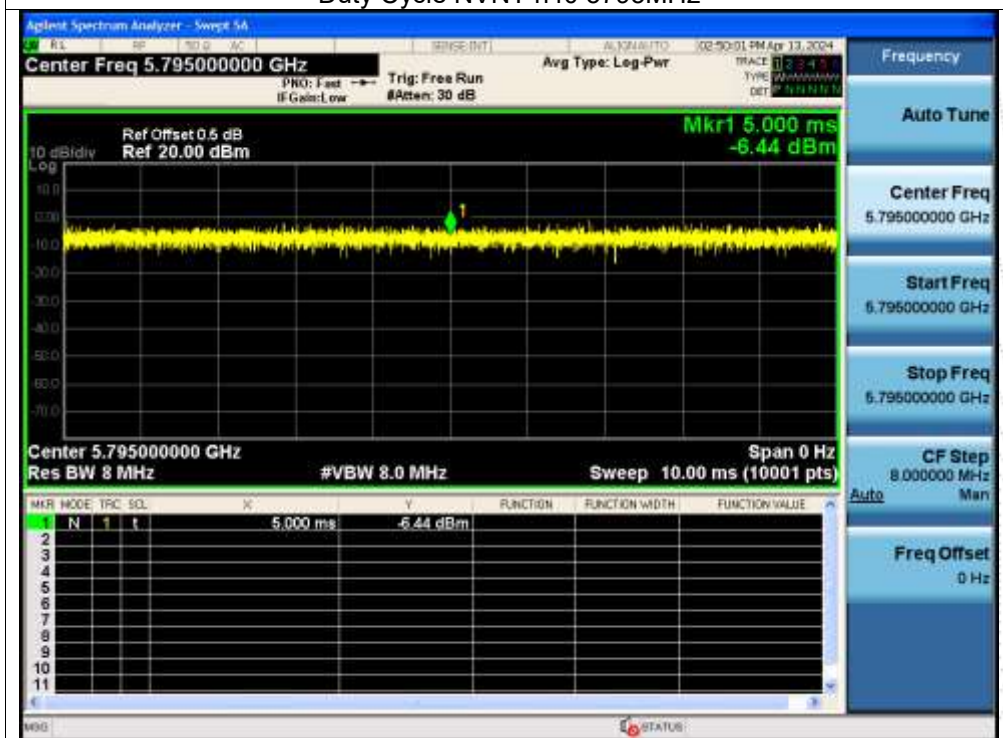
Duty Cycle NVNT n40 5795MHz
