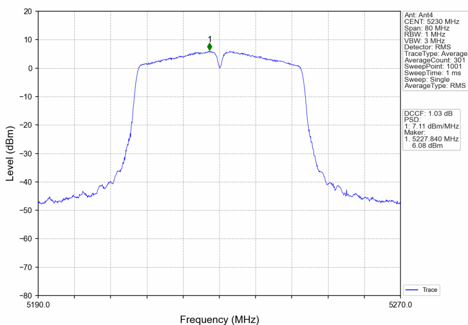
802.11ac(VHT40)_HCH_5230MHz_Ant4_NTNV
