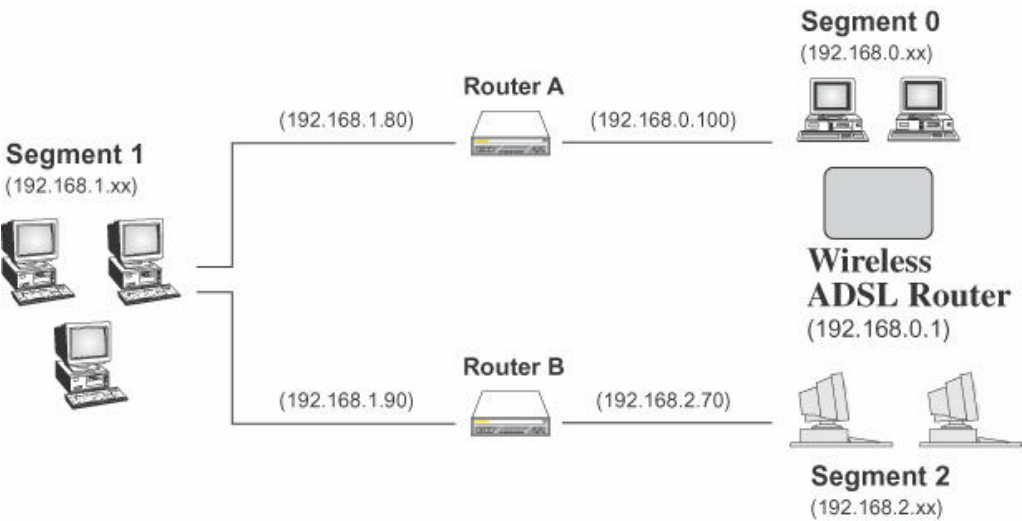
Figure 64: Routing Example
