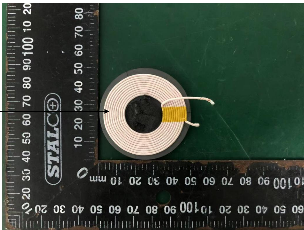
5W Coil Antenna
