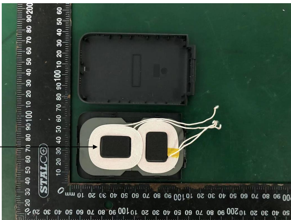
10W Coil Antenna
