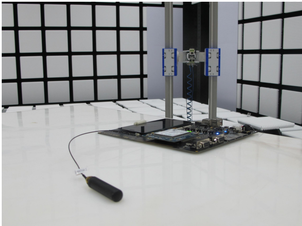
Pic7~8. Radiated emissions (26.5GHz-40GHz)
