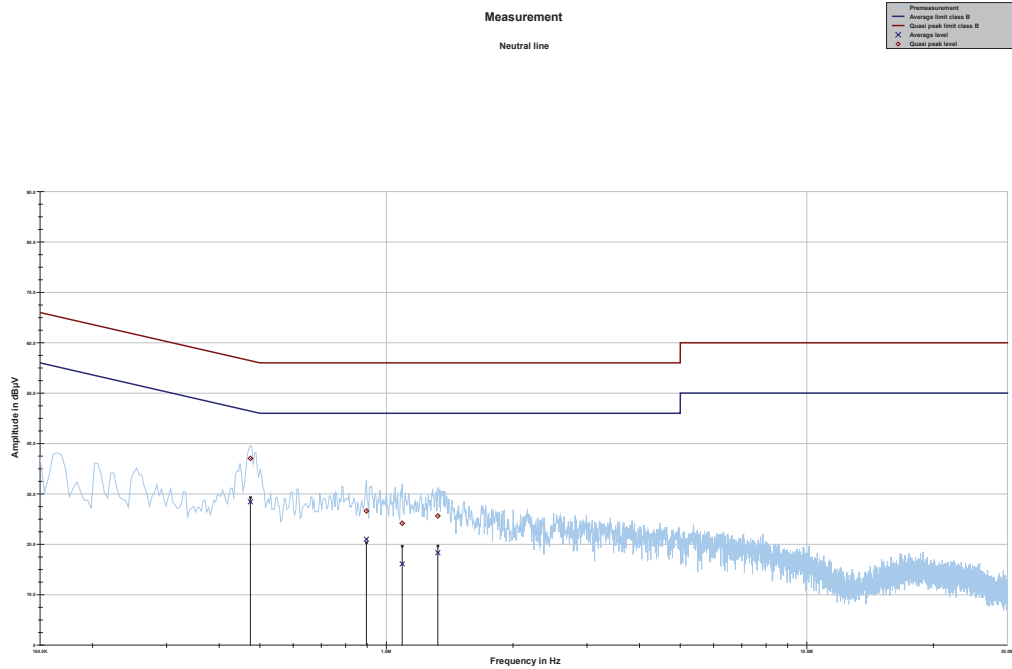
Plot 35: Neutral line
