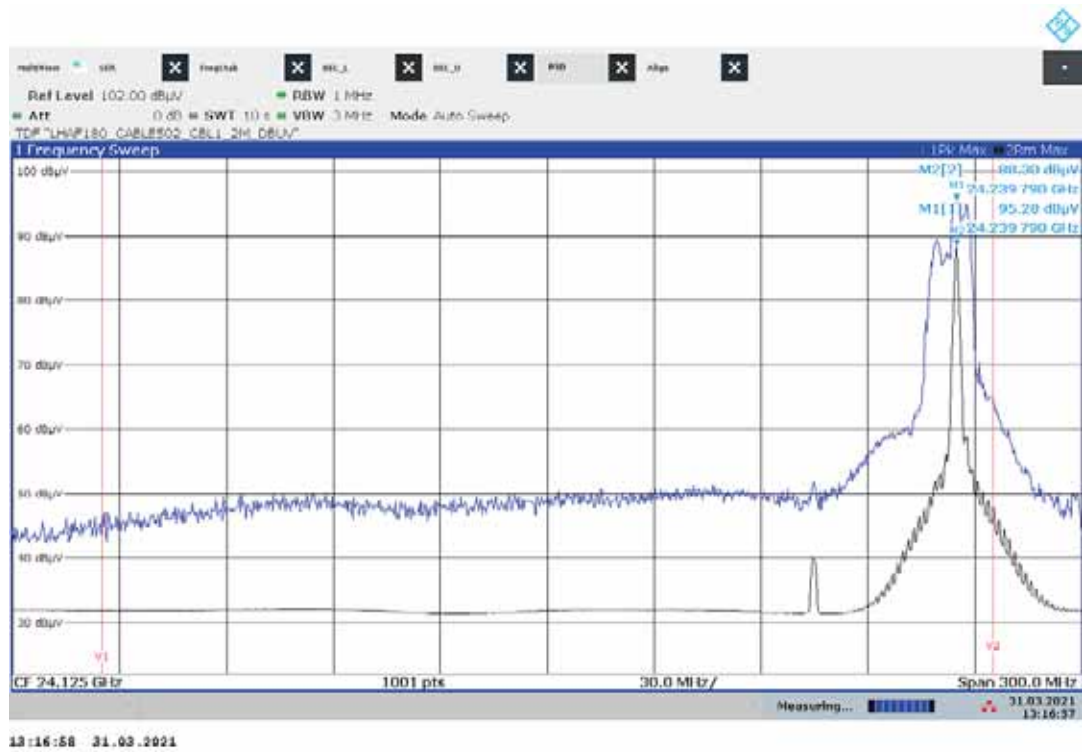
Plot No. 3: Field strength, f_{\text{high}}
