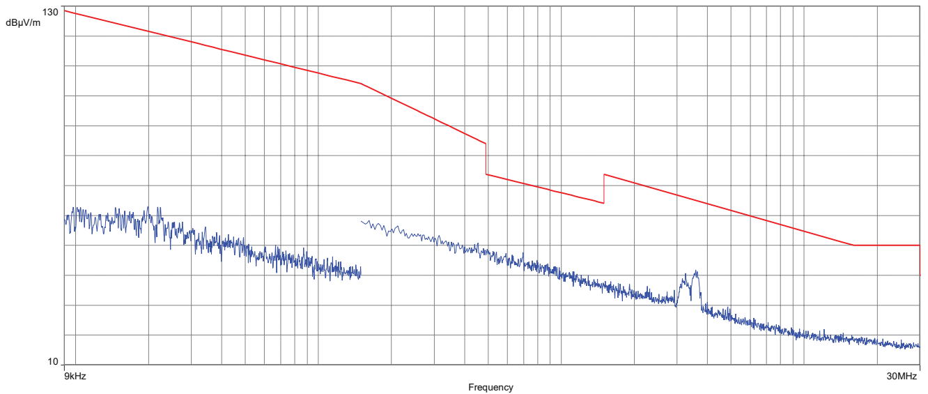
Plot No. 6: 9 kHz to 30 MHz, horizontal/vertical polarization, f_{\text{high}}
