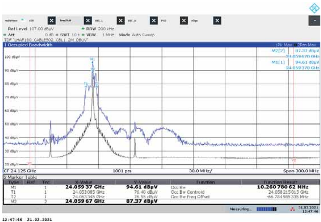
Plot 45: +20 °C, low frequency mode, V_{\text{nom}}
