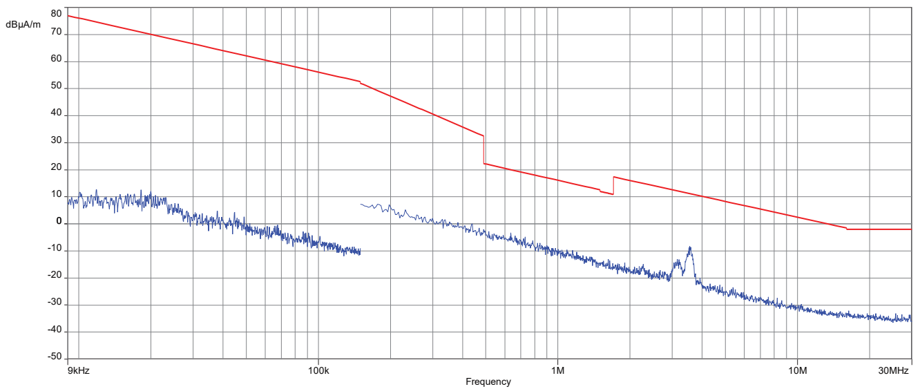
Plot No. 7: 9 kHz to 30 MHz, horizontal/vertical polarization, dBμA, f_{\text{low}}
