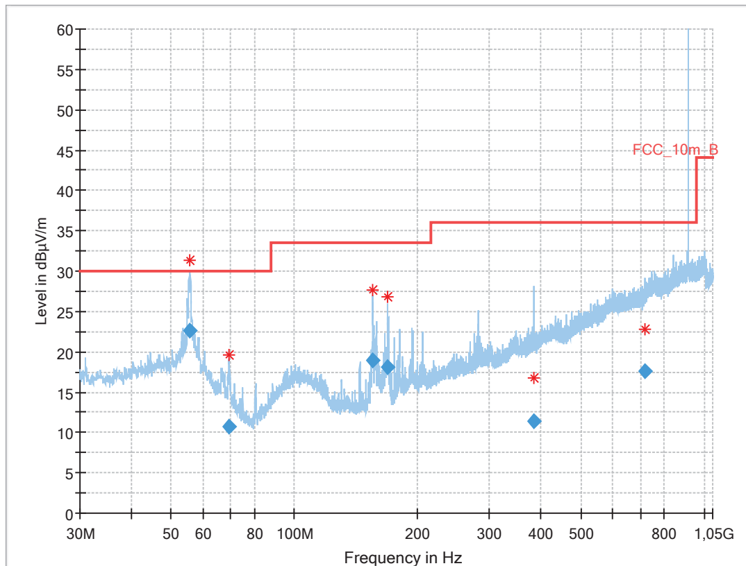
Plot No. 10: 30 MHz to 1 GHz, horizontal/vertical polarization, low channel
