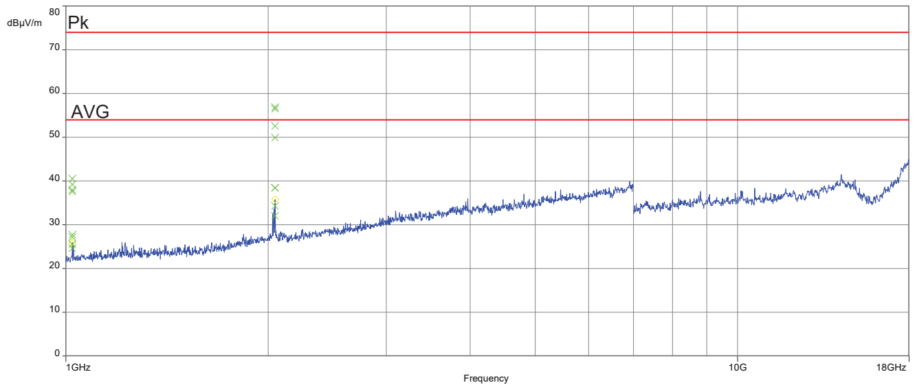
Plot No. 15: 1 GHz to 18 GHz, horizontal/vertical polarization, f_{\text{high}}
