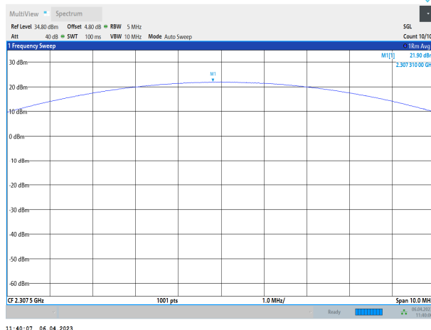
Band30-5MHz-QPSK-27685-1RB#12
