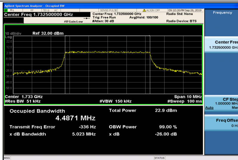
Band4-5MHz-16QAM-20175-25RB#0-4.4871
