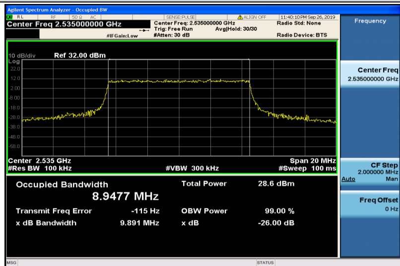
Band7-10MHz-QPSK-21100-50RB#0-8.9477
