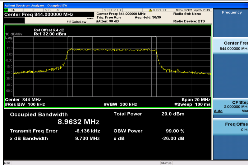
Band5-10MHz-QPSK-20600-50RB#0-8.9632
