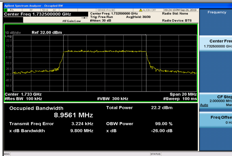
Band4-10MHz-16QAM-20175-50RB#0-8.9561
