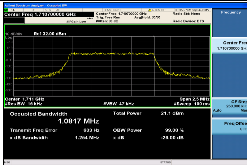
Band4-1.4MHz-16QAM-19957-6RB#0-1.0817
