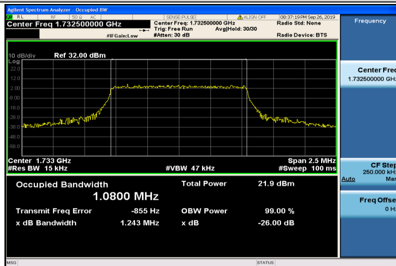
Band4-1.4MHz-QPSK-20175-6RB#0-1.0800
