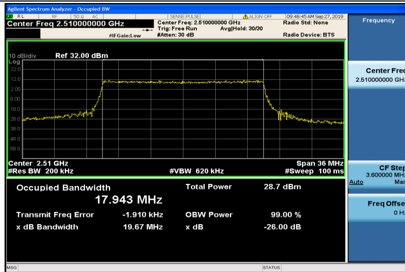
Band7-20MHz-QPSK-20850-100RB#0-17.943
