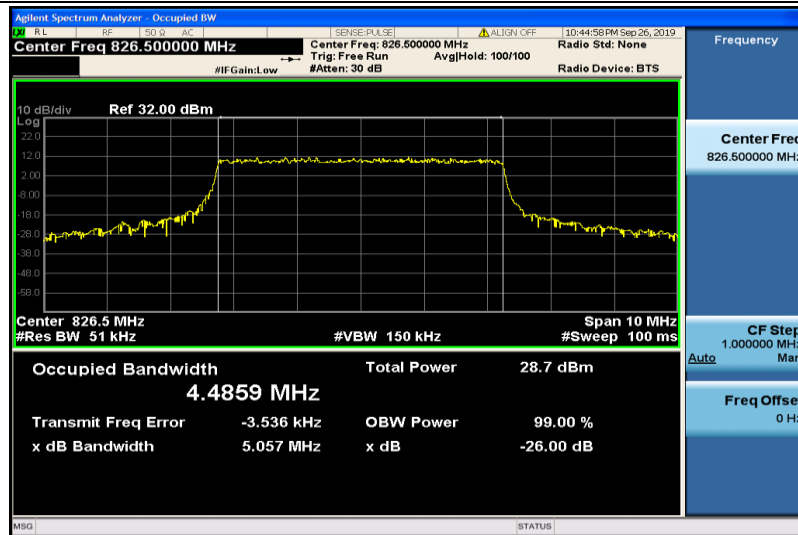
Band5-5MHz-QPSK-20425-25RB#0-4.4859
