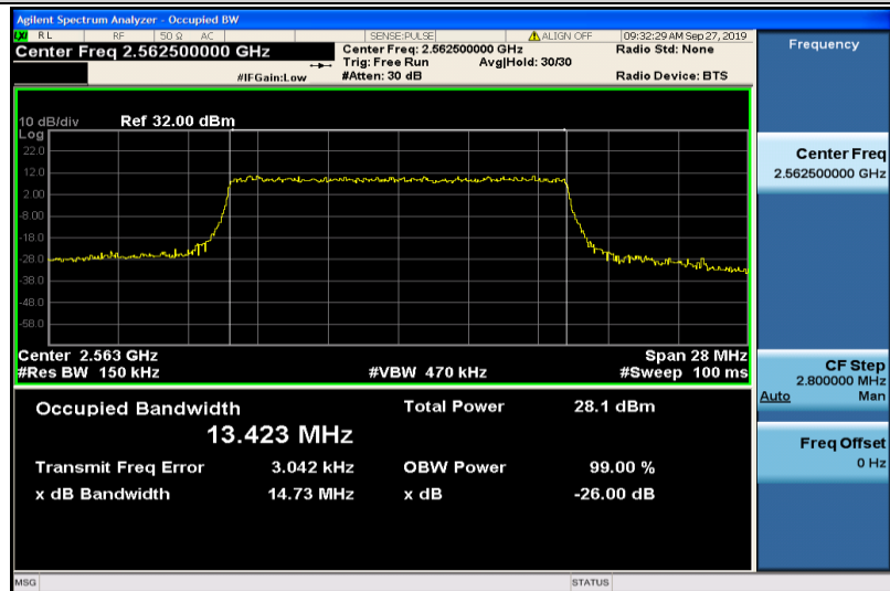
Band7-15MHz-16QAM-21375-75RB#0-13.423
