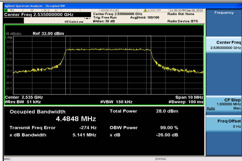
Band7-5MHz-16QAM-21100-25RB#0-4.4848
