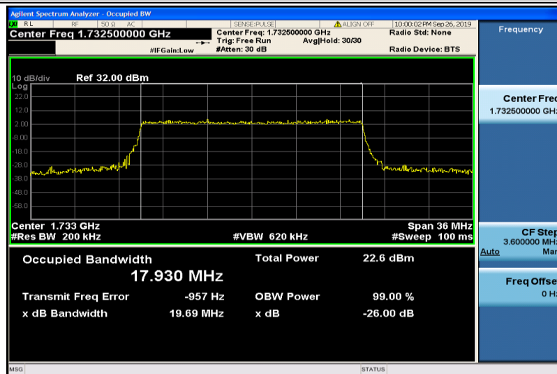
Band4-20MHz-16QAM-20175-100RB#0-17.930
