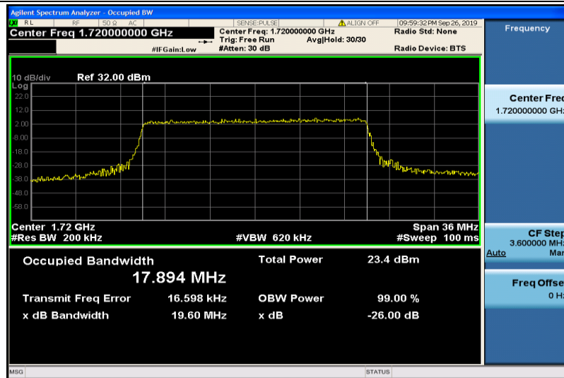
Band4-20MHz-QPSK-20050-100RB#0-17.894
