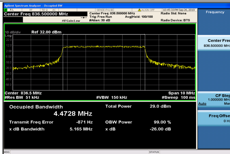
Band5-5MHz-QPSK-20525-25RB#0-4.4728
