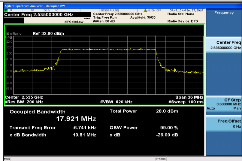
Band7-20MHz-16QAM-21100-100RB#0-17.921
