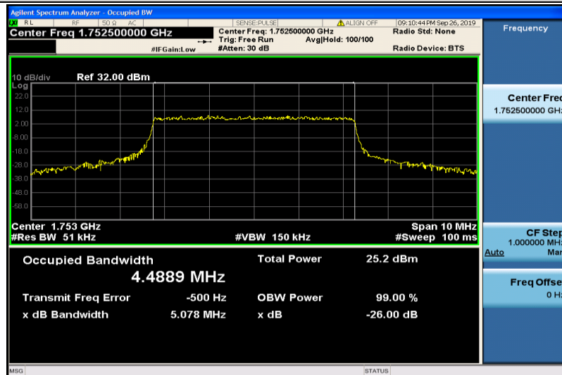
Band4-5MHz-QPSK-20375-25RB#0-4.4889
