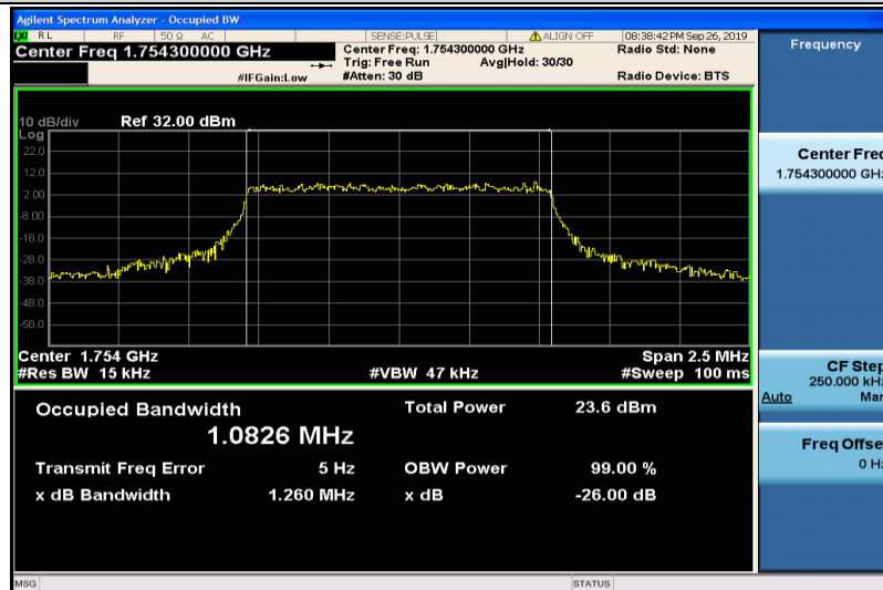
Band4-1.4MHz-QPSK-20393-6RB#0-1.0826
