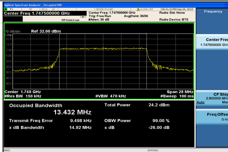
Band4-15MHz-QPSK-20325-75RB#0-13.432
