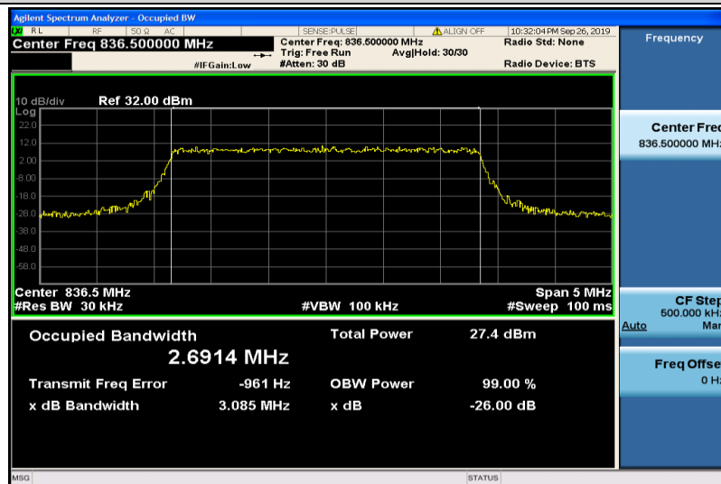
Band5-3MHz-16QAM-20525-15RB#0-2.6914
