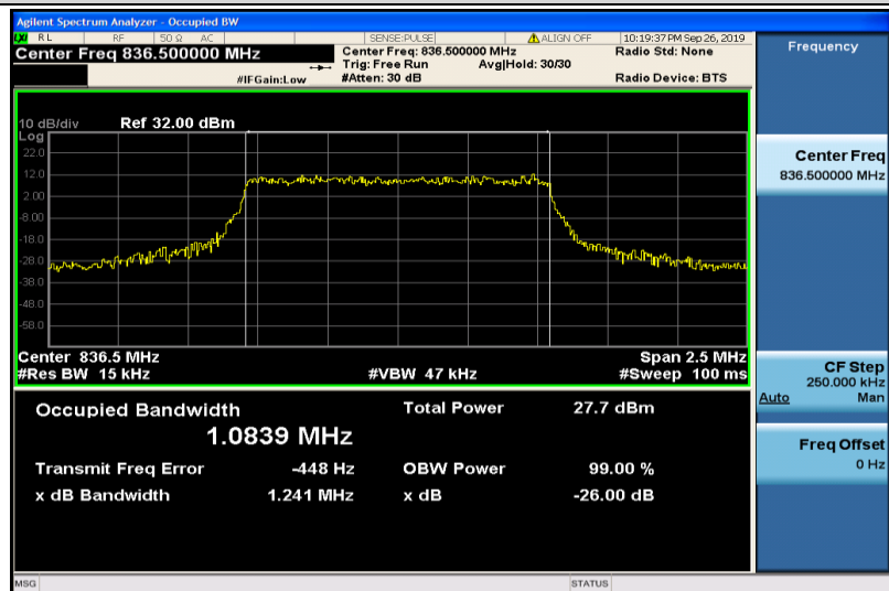
Band5-1.4MHz-QPSK-20525-6RB#0-1.0839
