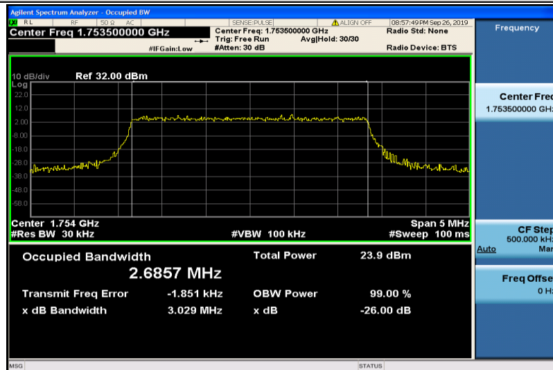
Band4-3MHz-16QAM-20385-15RB#0-2.6857
