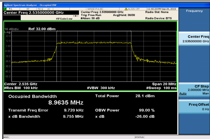
Band7-10MHz-16QAM-21100-50RB#0-8.9635
