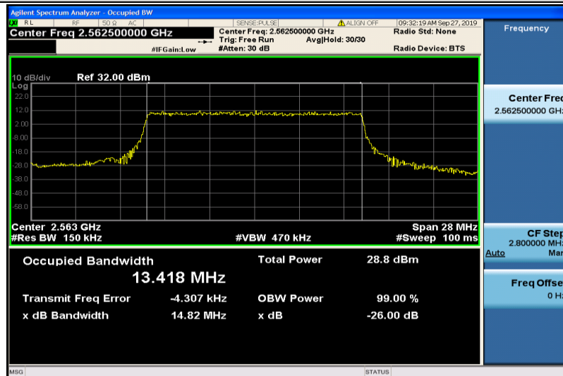
Band7-15MHz-QPSK-21375-75RB#0-13.418
