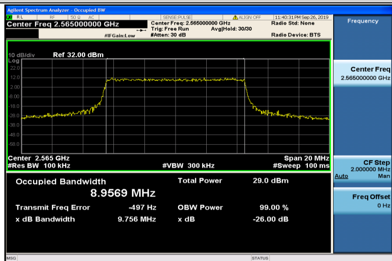
Band7-10MHz-QPSK-21400-50RB#0-8.9569
