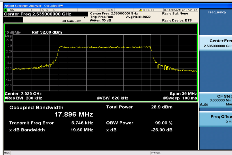
Band7-20MHz-QPSK-21100-100RB#0-17.896
