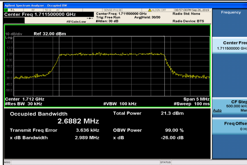
Band4-3MHz-16QAM-19965-15RB#0-2.6882
