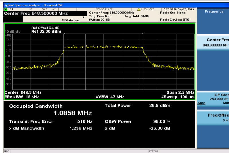
Band5-1.4MHz-16QAM-20643-6RB#0-1.0858
