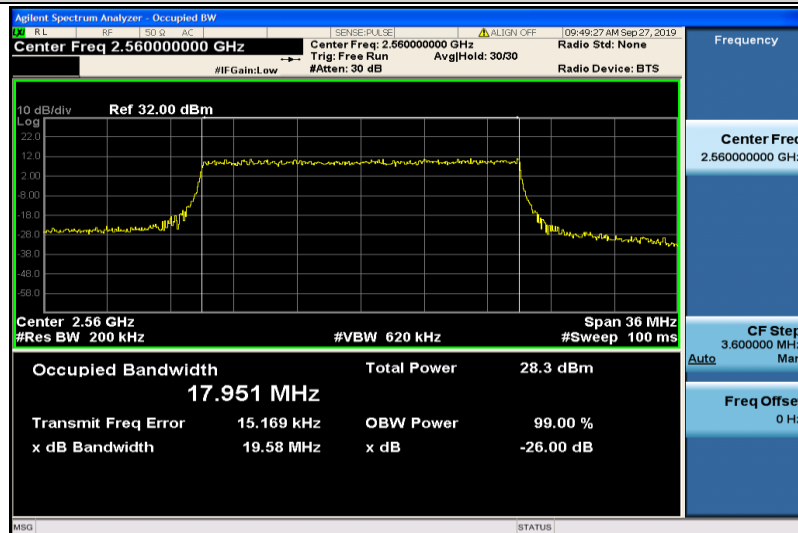
Band7-20MHz-QPSK-21350-100RB#0-17.951
