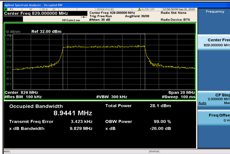
Band5-10MHz-16QAM-20450-50RB#0-8.9441
