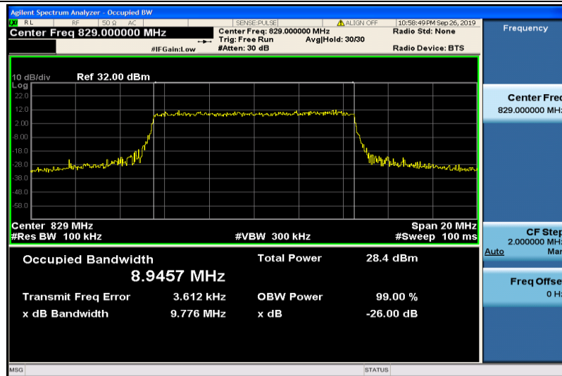
Band5-10MHz-QPSK-20450-50RB#0-8.9457
