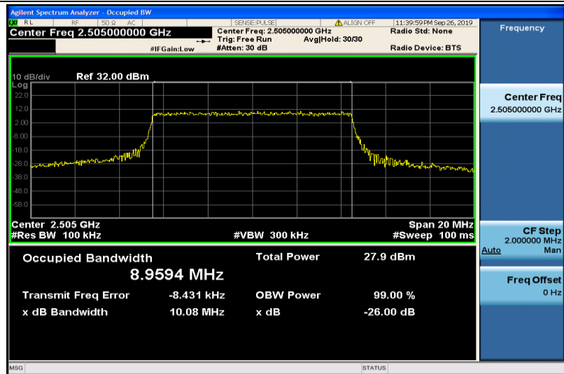
Band7-10MHz-16QAM-20800-50RB#0-8.9594
