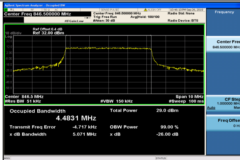
Band5-5MHz-QPSK-20625-25RB#0-4.4831
