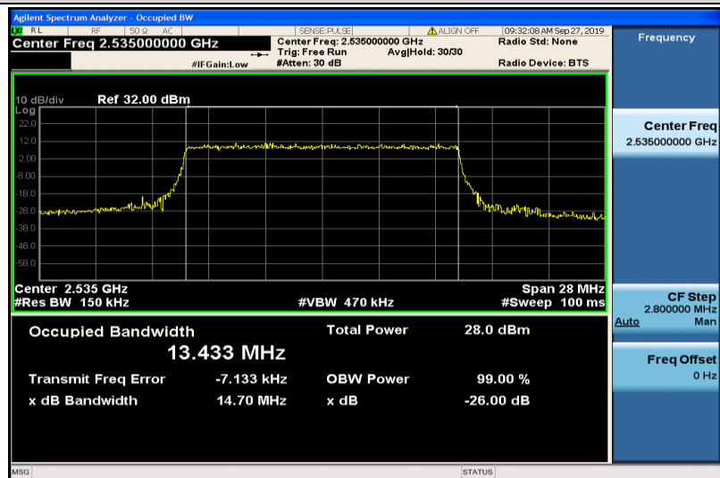
Band7-15MHz-16QAM-21100-75RB#0-13.433
