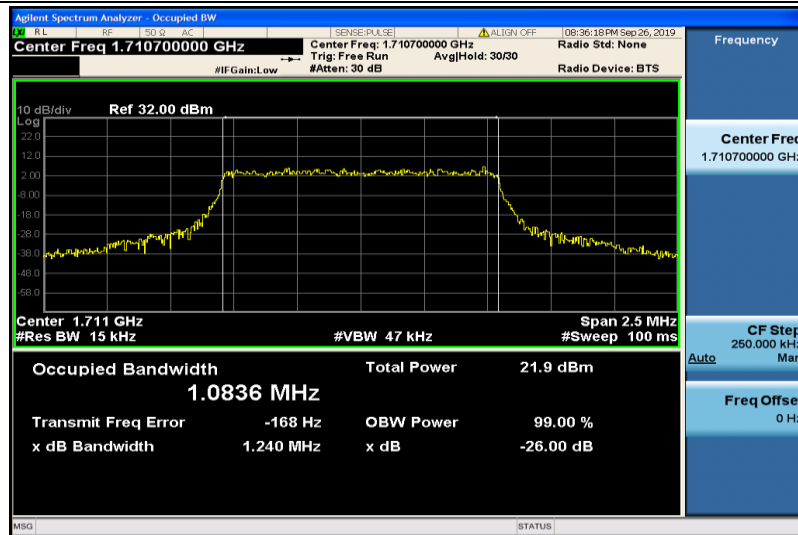
Band4-1.4MHz-QPSK-19957-6RB#0-1.0836
