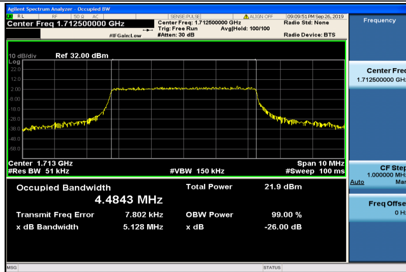
Band4-5MHz-16QAM-19975-25RB#0-4.4843
