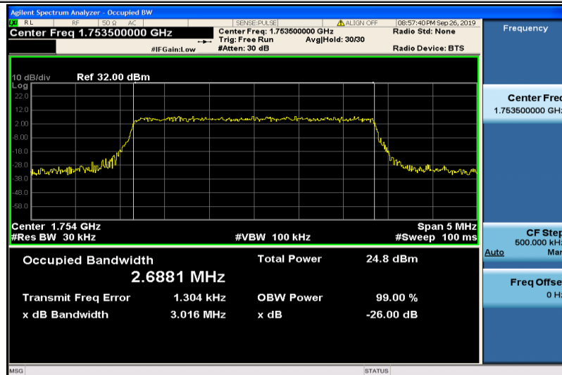
Band4-3MHz-QPSK-20385-15RB#0-2.6881
