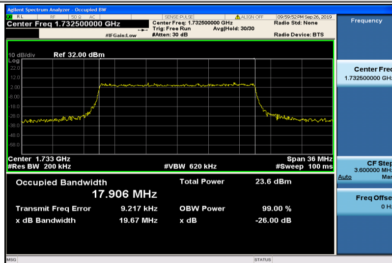
Band4-20MHz-QPSK-20175-100RB#0-17.906
