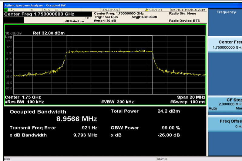
Band4-10MHz-QPSK-20350-50RB#0-8.9566
