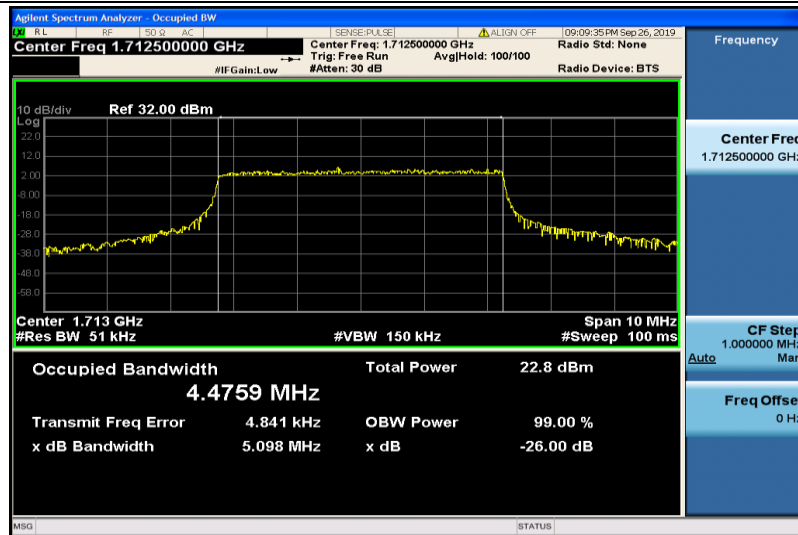
Band4-5MHz-QPSK-19975-25RB#0-4.4759
