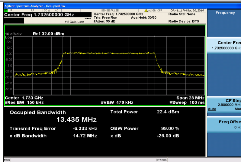
Band4-15MHz-16QAM-20175-75RB#0-13.435
