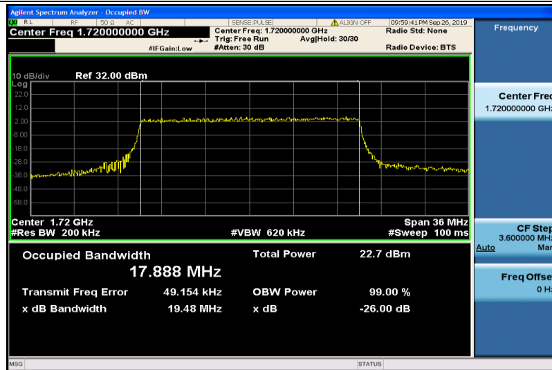
Band4-20MHz-16QAM-20050-100RB#0-17.888
