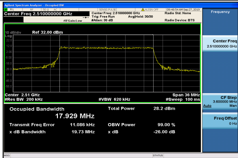
Band7-20MHz-16QAM-20850-100RB#0-17.929
