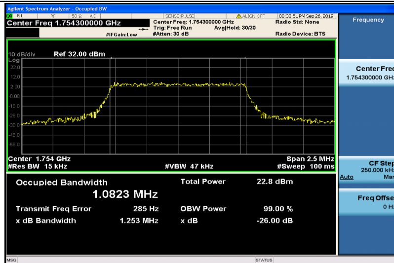
Band4-1.4MHz-16QAM-20393-6RB#0-1.0823
