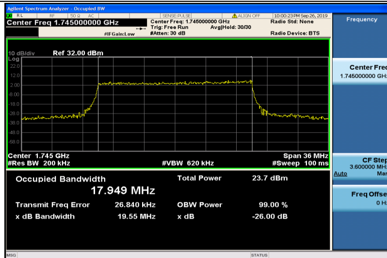
Band4-20MHz-16QAM-20300-100RB#0-17.949
