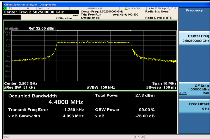
Band7-5MHz-16QAM-20775-25RB#0-4.4808
