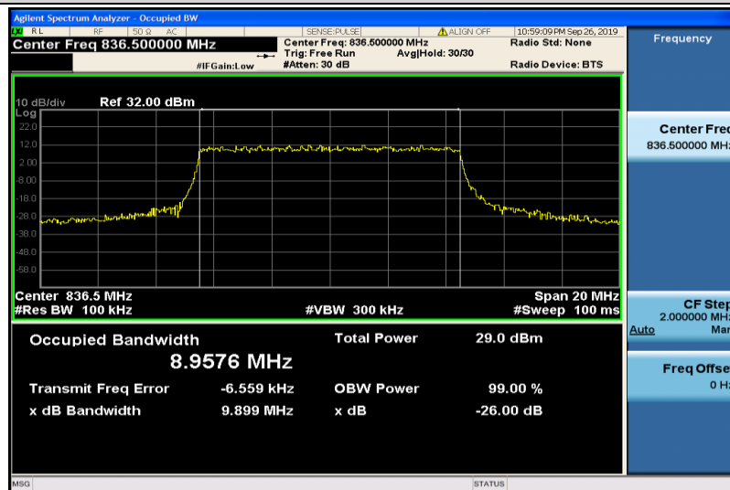
Band5-10MHz-QPSK-20525-50RB#0-8.9576
