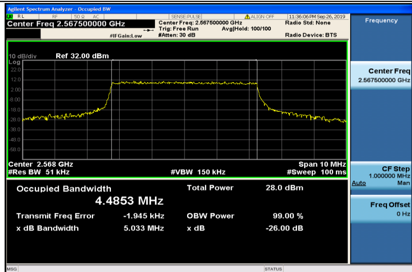
Band7-5MHz-16QAM-21425-25RB#0-4.4853
