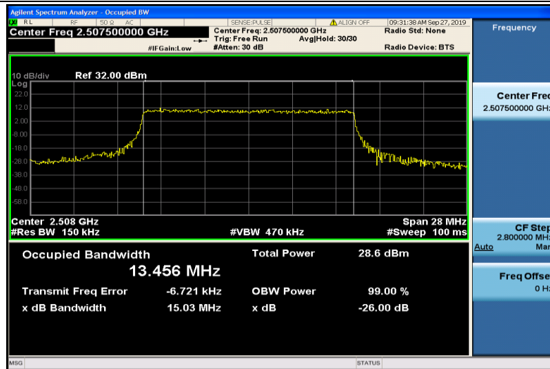
Band7-15MHz-QPSK-20825-75RB#0-13.456
