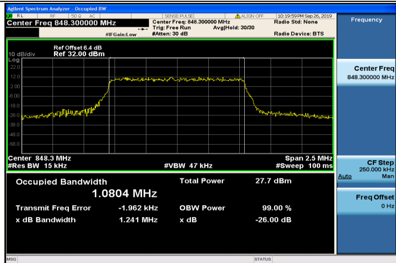
Band5-1.4MHz-QPSK-20643-6RB#0-1.0804
