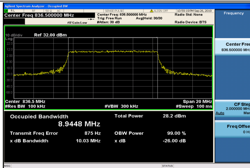
Band5-10MHz-16QAM-20525-50RB#0-8.9448
