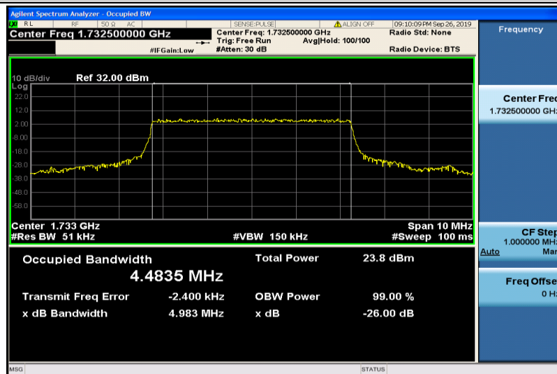
Band4-5MHz-QPSK-20175-25RB#0-4.4835
