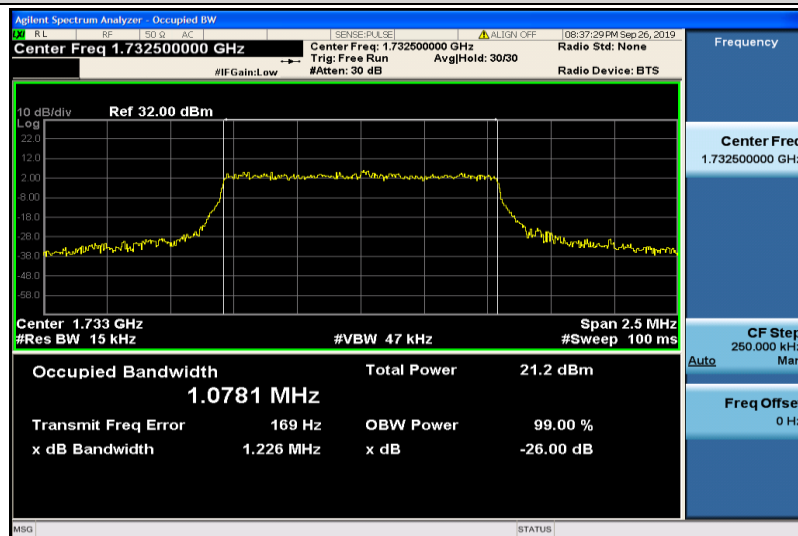
Band4-1.4MHz-16QAM-20175-6RB#0-1.0781
