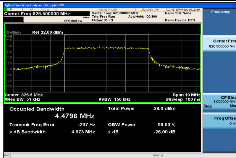
Band5-5MHz-16QAM-20425-25RB#0-4.4796
