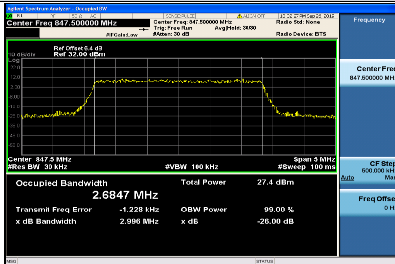
Band5-3MHz-16QAM-20635-15RB#0-2.6847
