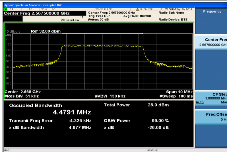
Band7-5MHz-QPSK-21425-25RB#0-4.4791
