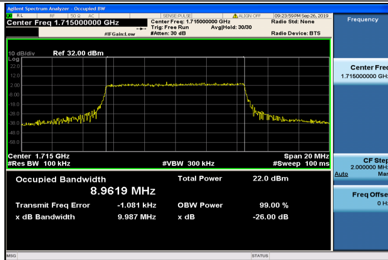
Band4-10MHz-16QAM-20000-50RB#0-8.9619
