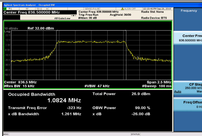
Band5-1.4MHz-16QAM-20525-6RB#0-1.0824
