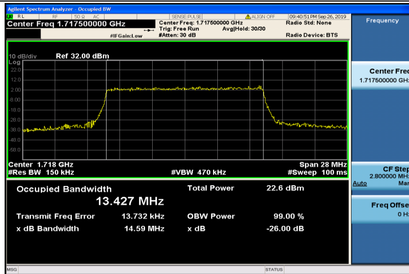
Band4-15MHz-16QAM-20025-75RB#0-13.427
