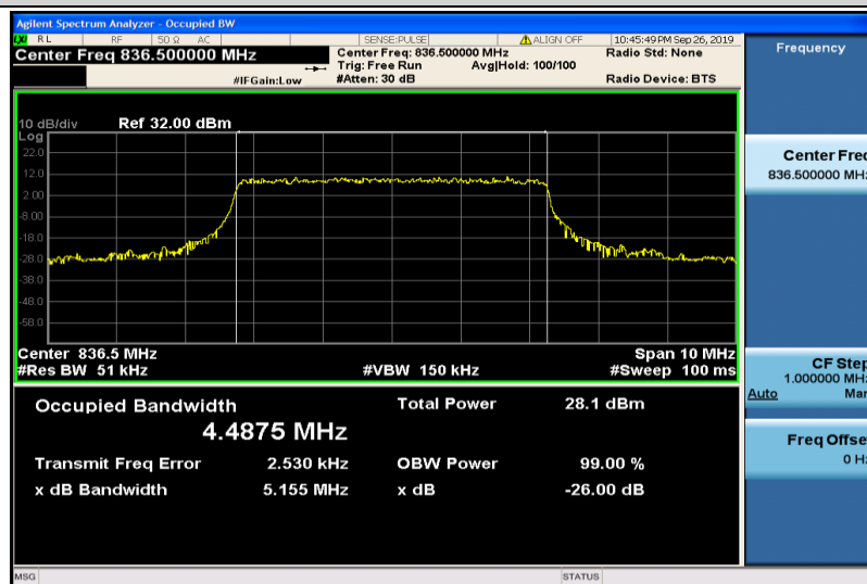
Band5-5MHz-16QAM-20525-25RB#0-4.4875
