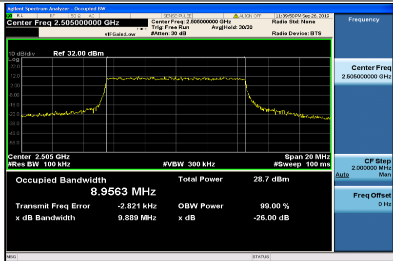
Band7-10MHz-QPSK-20800-50RB#0-8.9563
