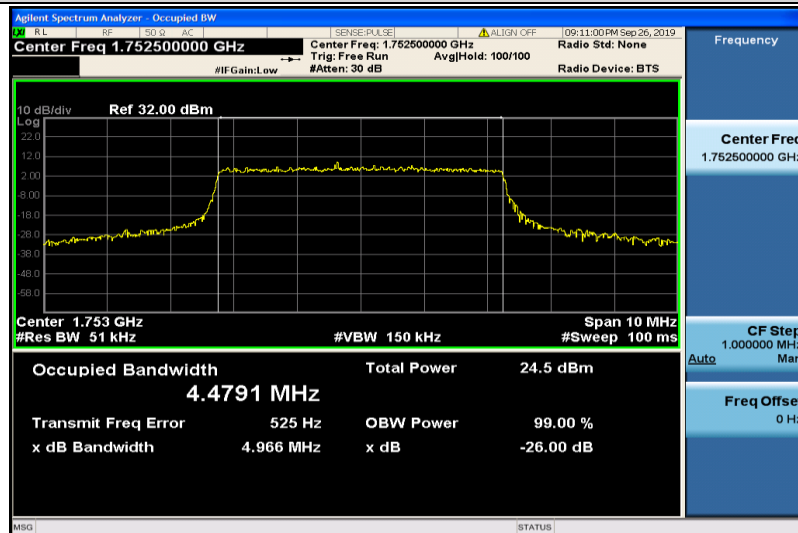
Band4-5MHz-16QAM-20375-25RB#0-4.4791
