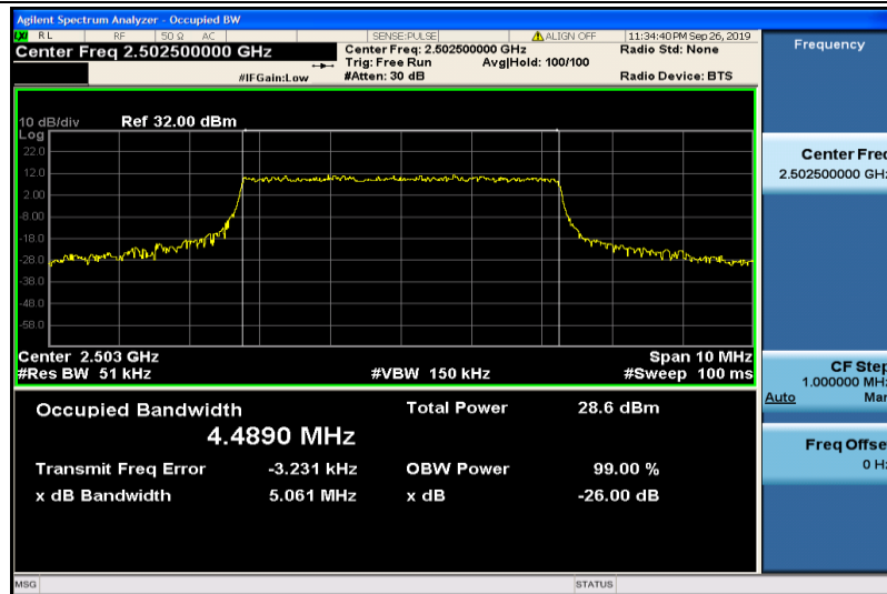
Band7-5MHz-QPSK-20775-25RB#0-4.4890
