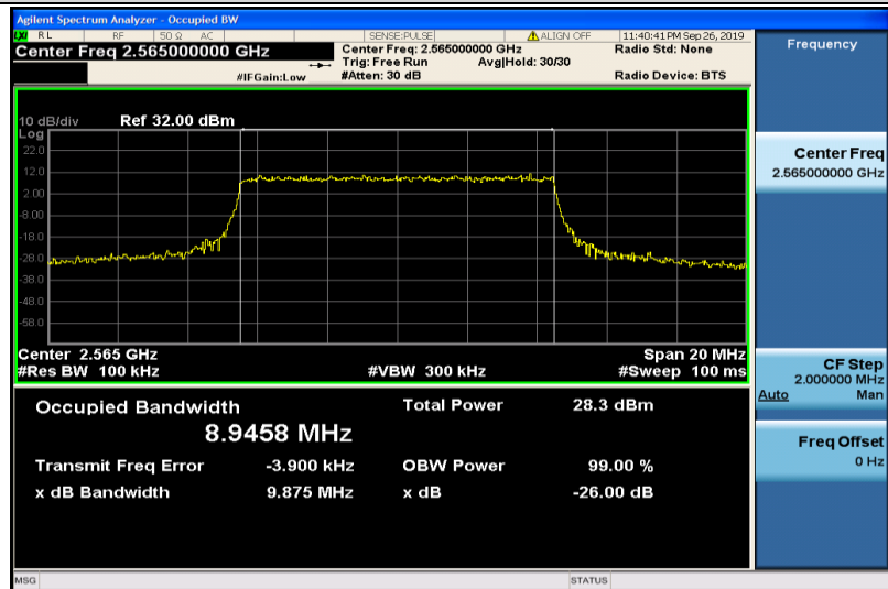
Band7-10MHz-16QAM-21400-50RB#0-8.9458
