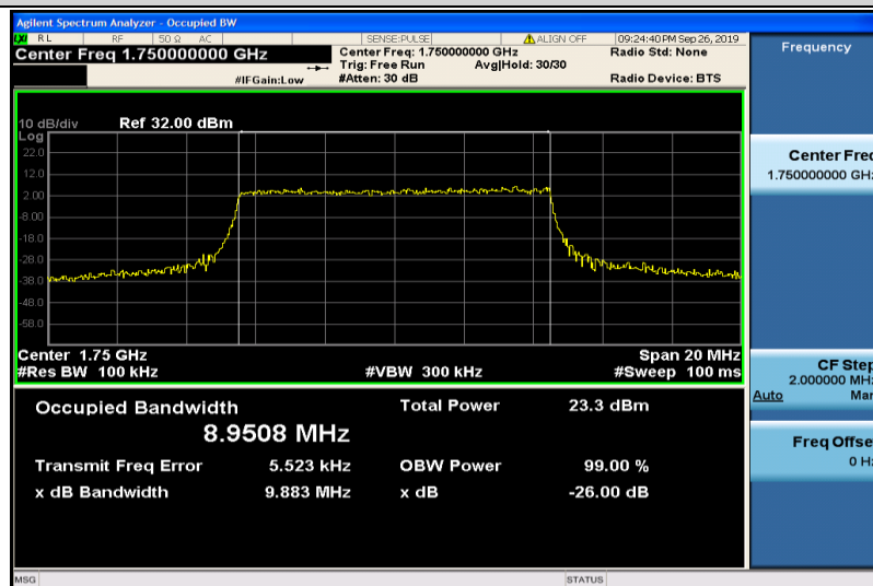
Band4-10MHz-16QAM-20350-50RB#0-8.9508
