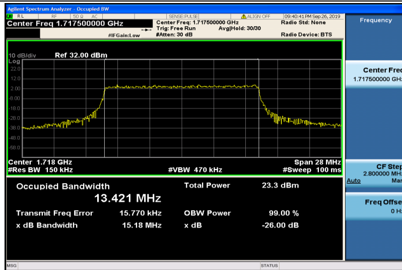
Band4-15MHz-QPSK-20025-75RB#0-13.421
