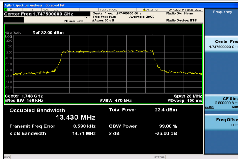
Band4-15MHz-16QAM-20325-75RB#0-13.430
