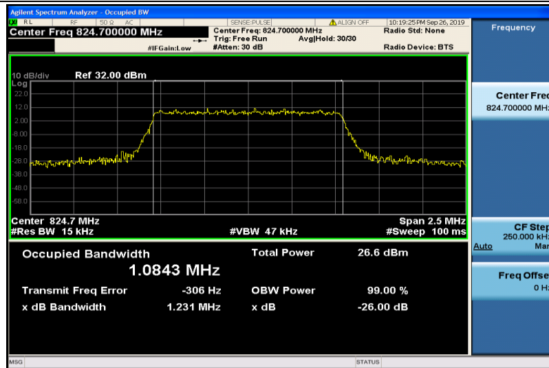
Band5-1.4MHz-16QAM-20407-6RB#0-1.0843
