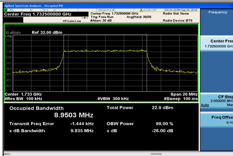
Band4-10MHz-QPSK-20175-50RB#0-8.9503
