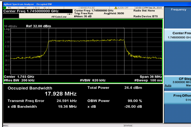
Band4-20MHz-QPSK-20300-100RB#0-17.928
