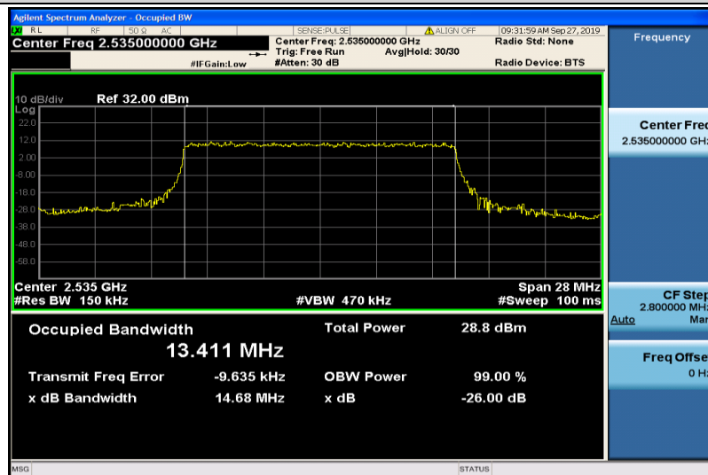
Band7-15MHz-QPSK-21100-75RB#0-13.411
