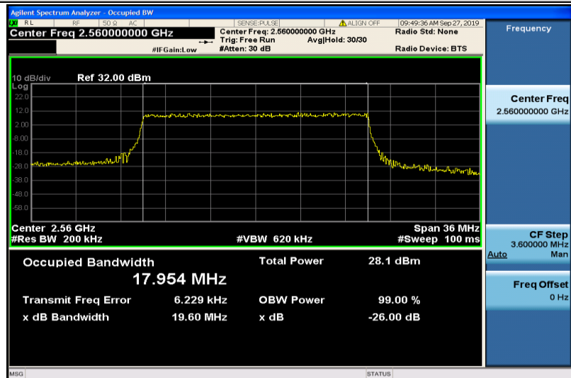
Band7-20MHz-16QAM-21350-100RB#0-17.954
