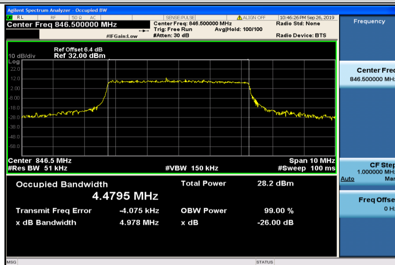
Band5-5MHz-16QAM-20625-25RB#0-4.4795
