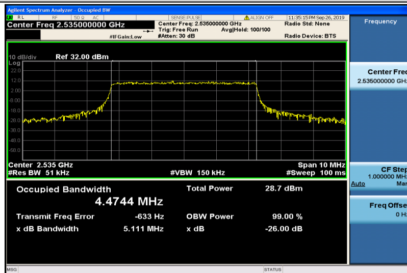
Band7-5MHz-QPSK-21100-25RB#0-4.4744
