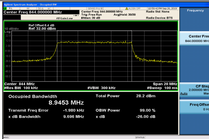
Band5-10MHz-16QAM-20600-50RB#0-8.9453
