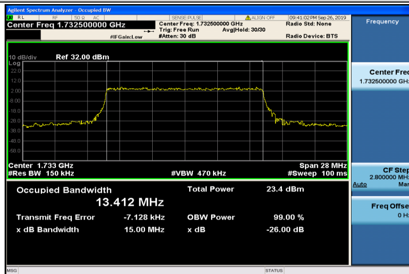
Band4-15MHz-QPSK-20175-75RB#0-13.412
