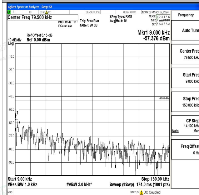
Band2_5MHz_QPSK_18900_1RB#0_0.009~0.15_0.009~ 0.15
