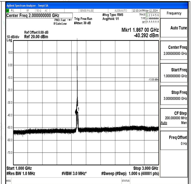
Band2_5MHz_QPSK_18900_1RB#0_1000~3000_1000~3000
