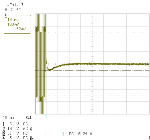
Plot 7.7.4 Transient frequency during power OFF test results at mid carrier frequency
