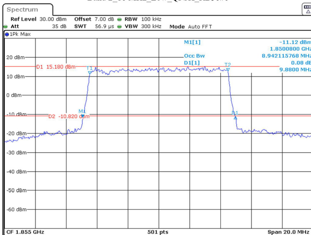
Band 2 10 MHz Low QPSK RB50#0
