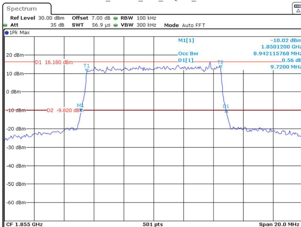
Band 2 10 MHz Low 16QAM RB50#0
