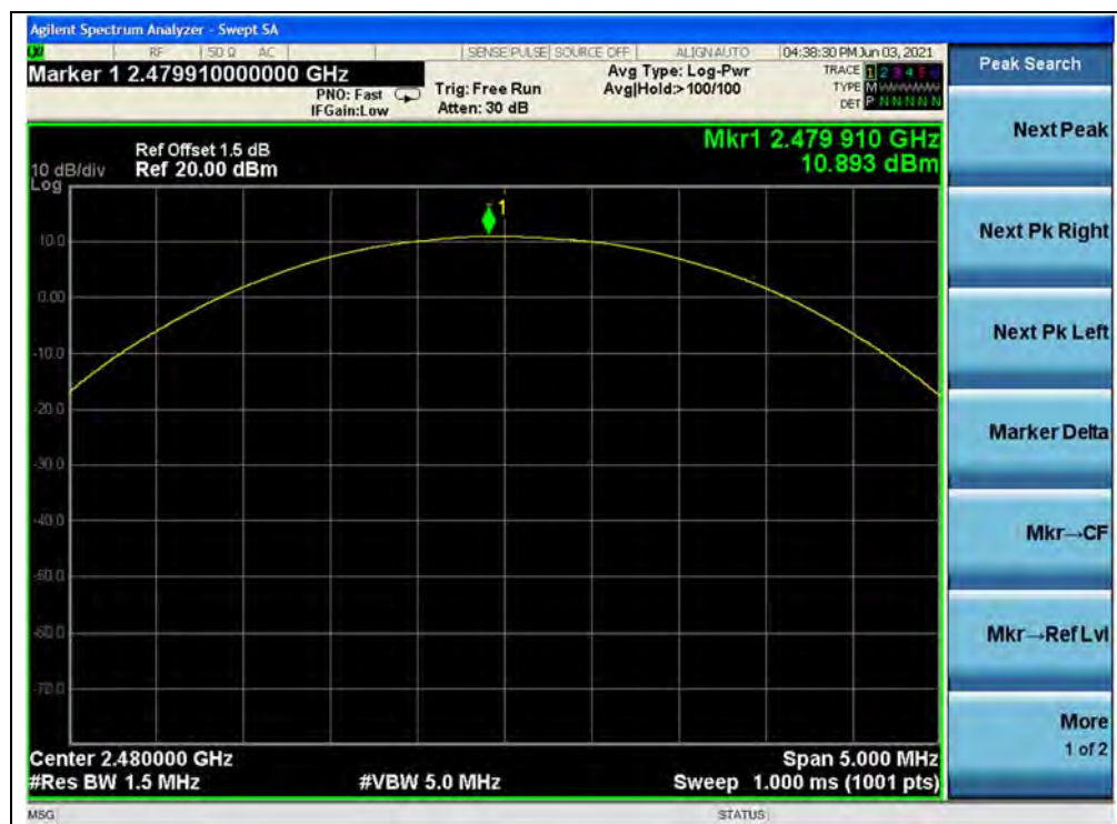
(Channel 78, 8-DPSK)
