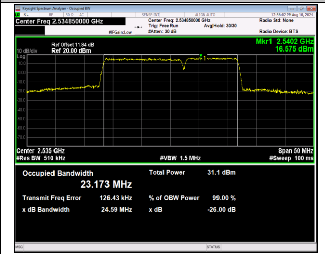
7-7-15MHz-10MHz-QPSK-QPSK-21051-21171-75RB#0-5 ORB#0-PASS
