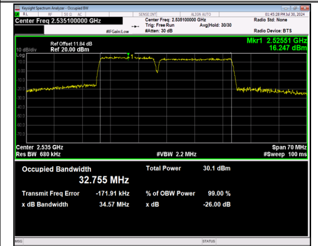
7-7-15MHz-20MHz-64QAM-64QAM-21003-21174-75RB#0 -100RB#0-PASS
