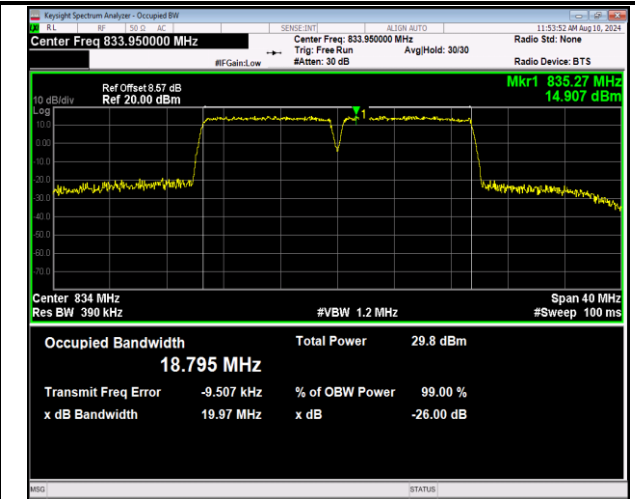
5-5-10MHz-10MHz-16QAM-16QAM-20450-20549-50RB#0-5 -50RB#0-PASS
