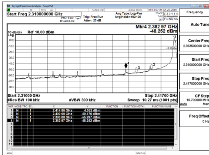
Channel 0 / 2415 MHz
