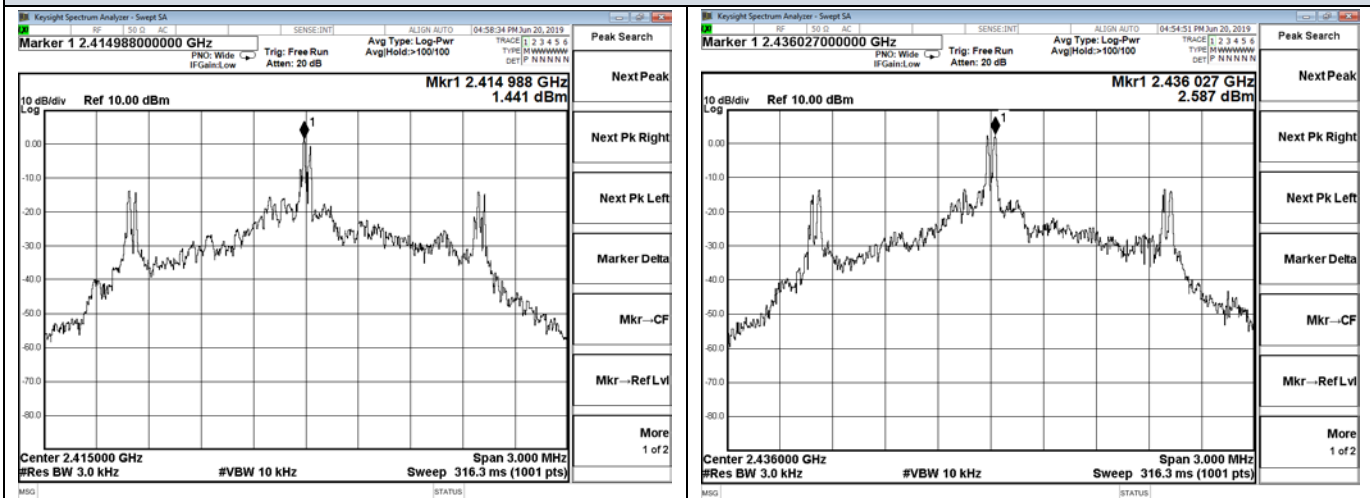
Channel 0 / 2415 MHz
