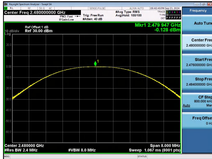
BLE_1M-Ant1-2480-PASS
