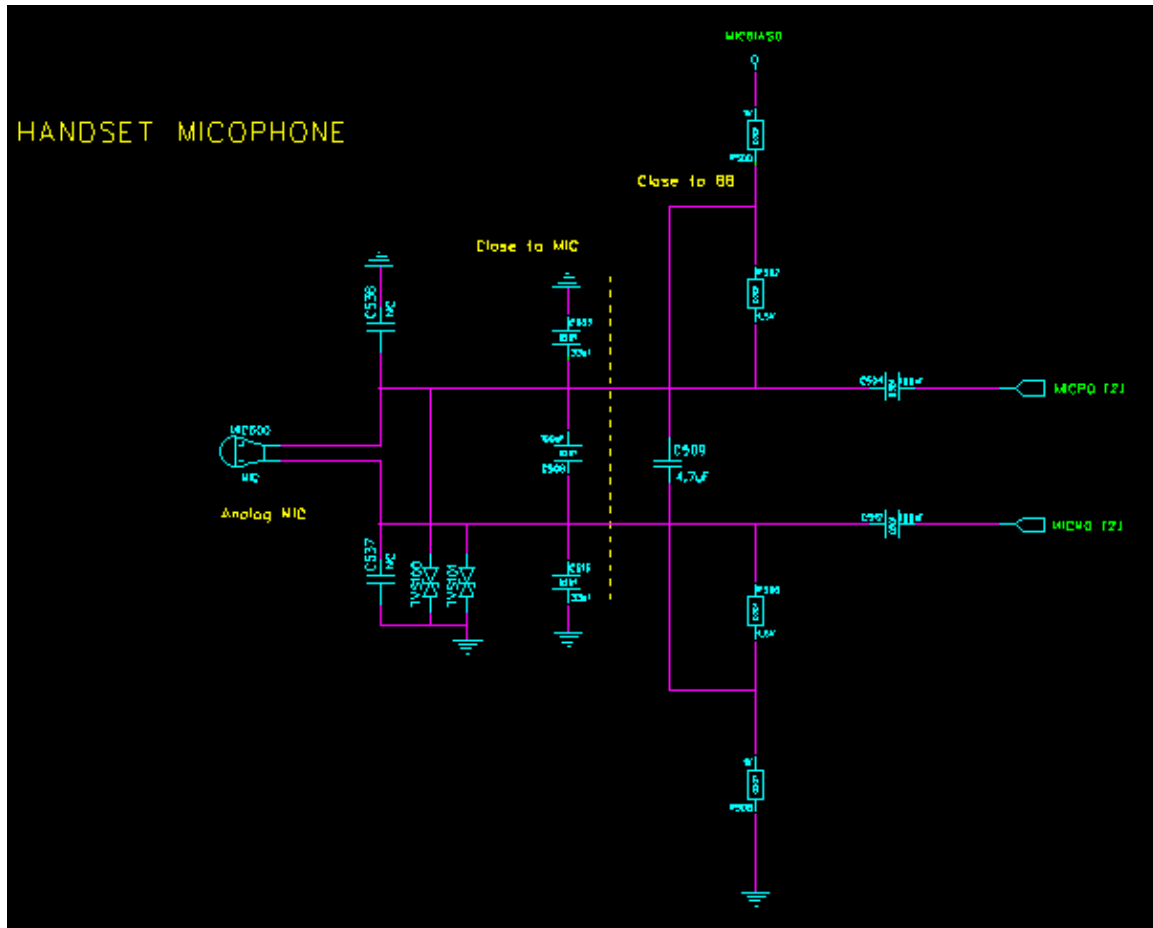
Figure 3.2.1 Micphone circuit
