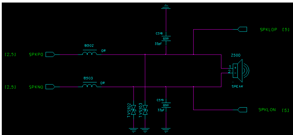
Figure 3.2.3: Speaker circuit
