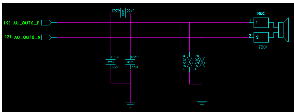
Figure 3.2.2 Receiver circuit
