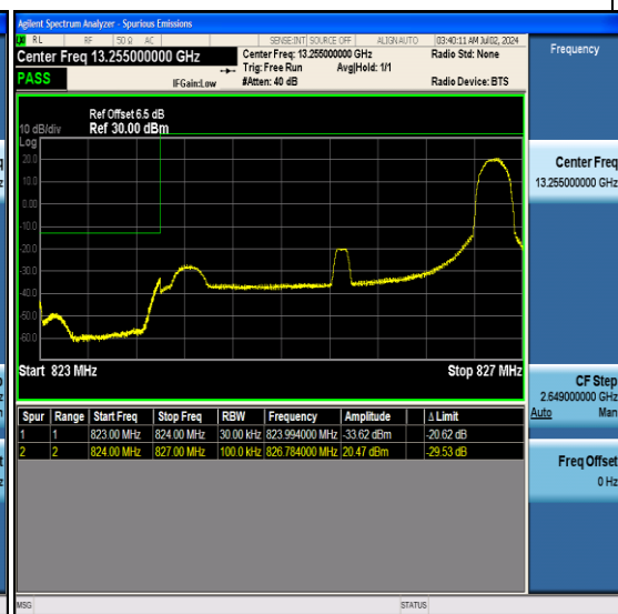
Band5_3MHz_16QAM_20415_1RB#14
