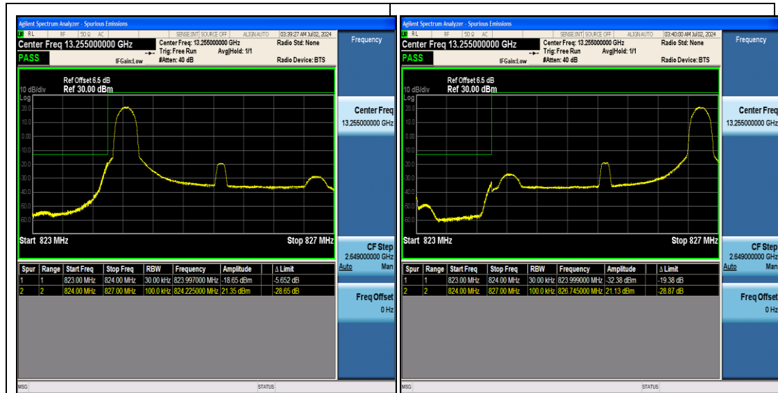
Band5_3MHz_QPSK_20415_1RB#0
