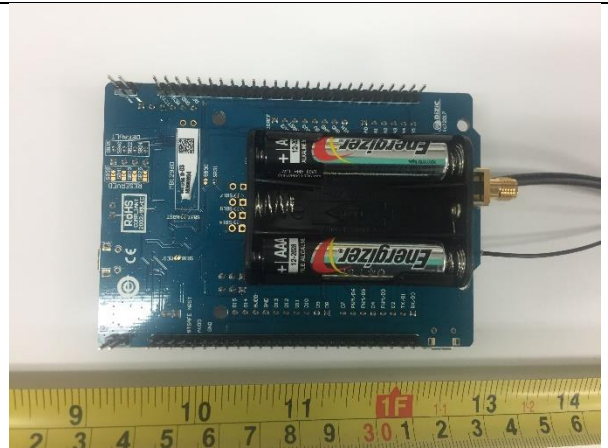
EUT on development board Bottom View
