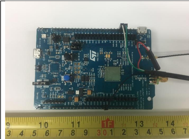
EUT on development board Top View
