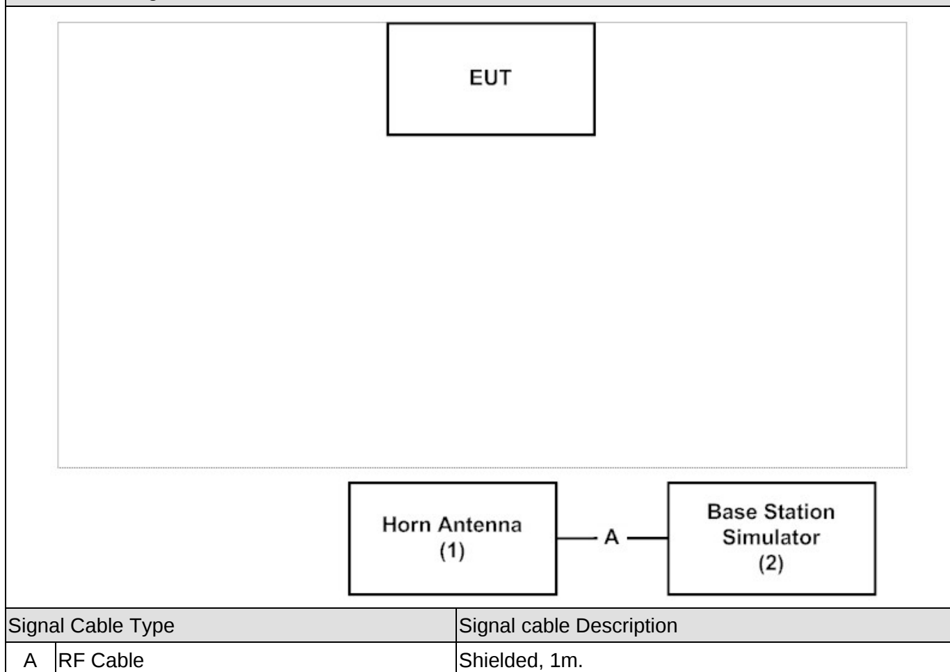
Connection Diagram
