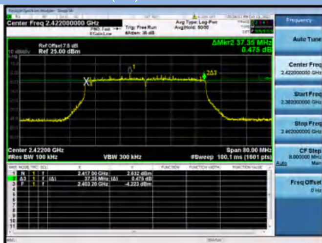
802.11ax-40 MHz(SU)CHANNEL 3
