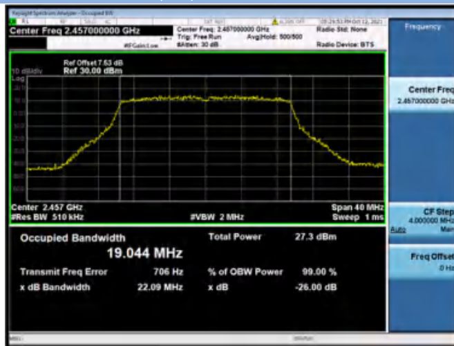
802.11ax-20 MHz(SU)CHANNEL 10
