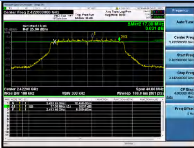
802.11ax-20 MHz(SU)CHANNEL 3
