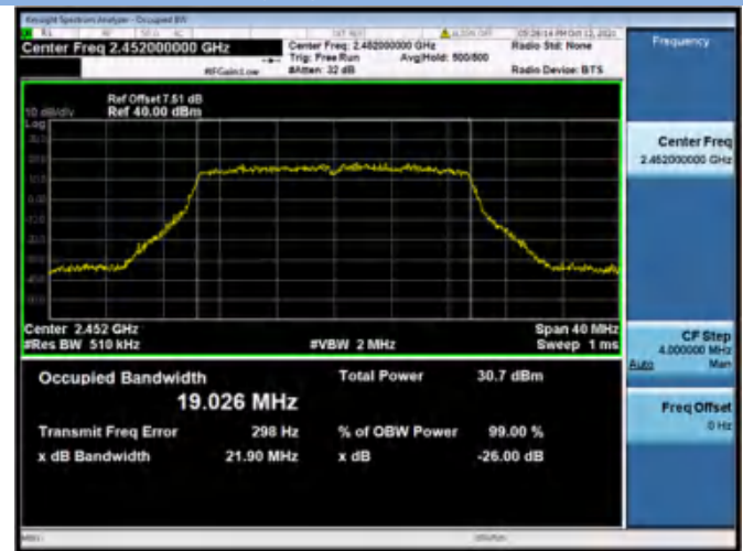
802.11ax-20 MHz(SU) CHANNEL 9
