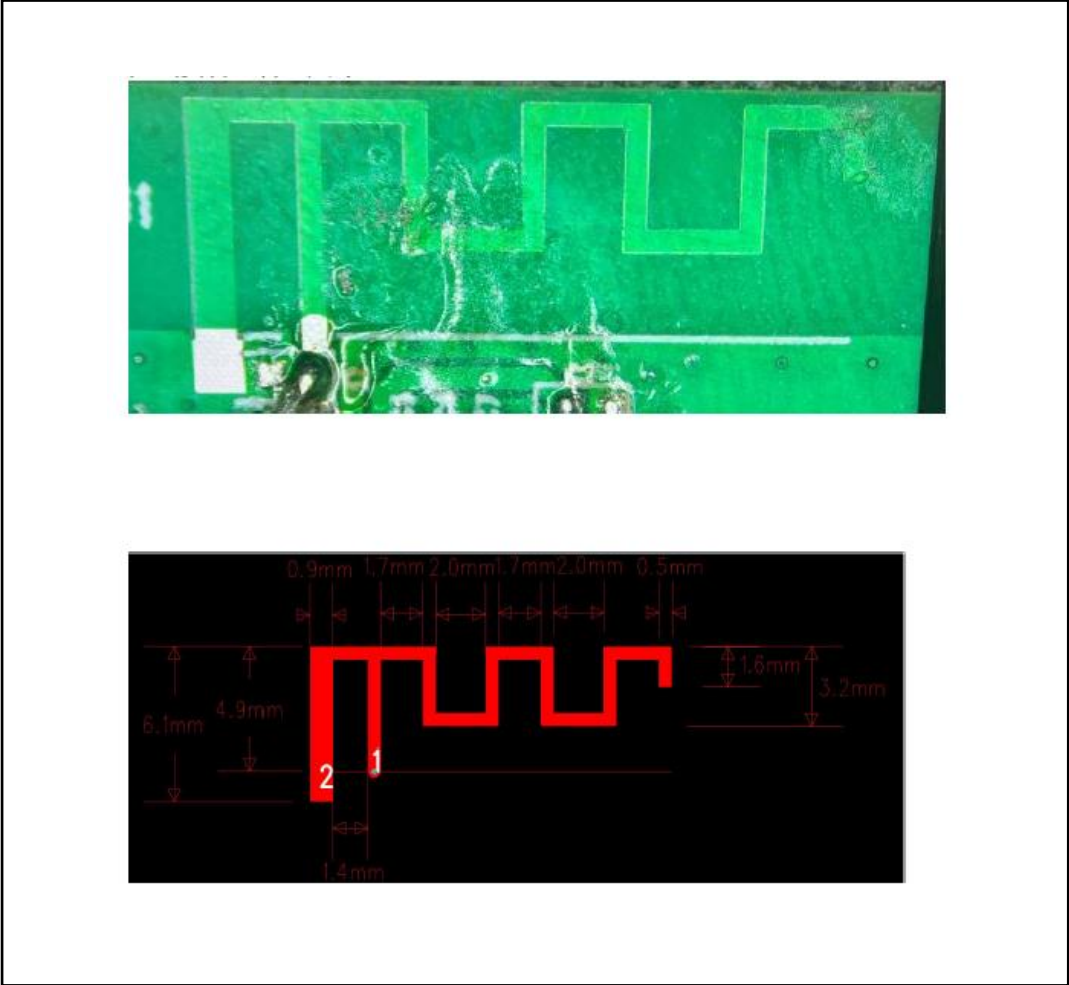
产品规格图(Antenna Specification chart)
