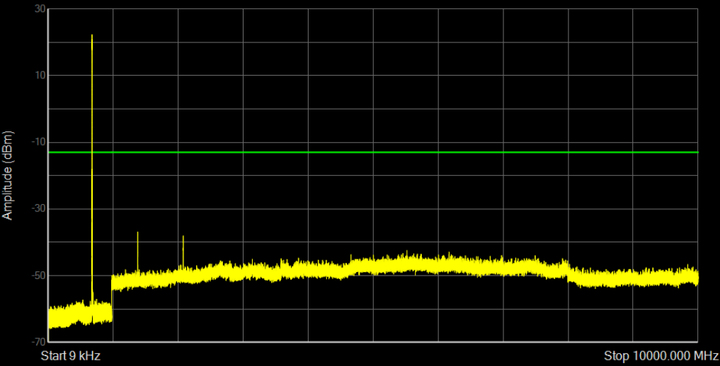
Band12 QAM16 BW=1.4MHz Channel=23017 RB Size=6 Position=#0
