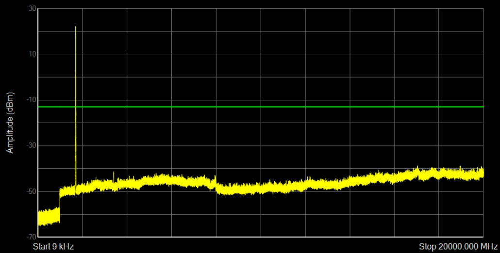
Band66 QPSK BW=5MHz Channel=131997 RB Size=25 Position=#0
