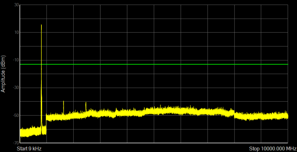
Band5 QAM16 BW=5MHz Channel=20425 RB Size=25 Position=#0
