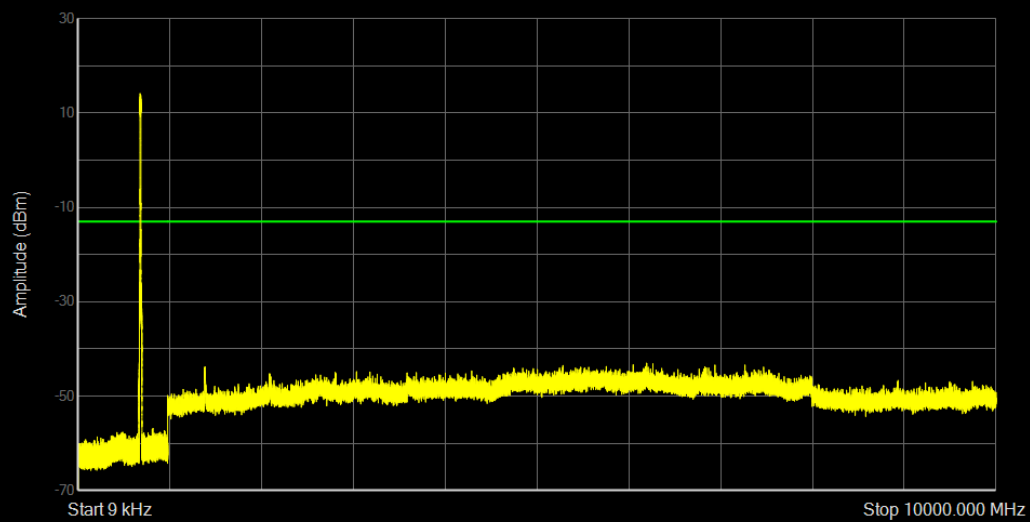
Band12 QPSK BW=10MHz Channel=23060 RB Size=50 Position=#0
