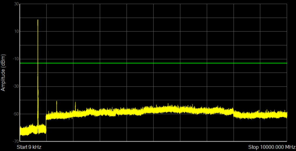
Band12 QPSK BW=3MHz Channel=23025 RB Size=15 Position=#0
