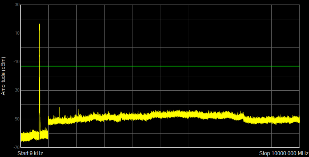
Band12 QPSK BW=5MHz Channel=23035 RB Size=25 Position=#0
