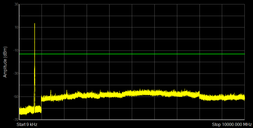
Band12 QPSK BW=10MHz Channel=23130 RB Size=50 Position=#0
