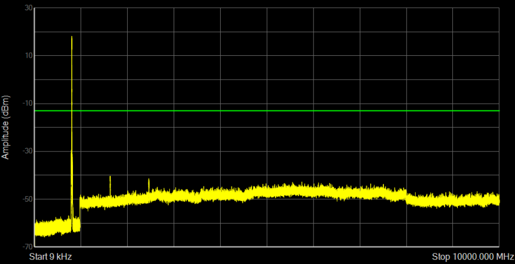
Band5 QPSK BW=5MHz Channel=20425 RB Size=25 Position=#0
