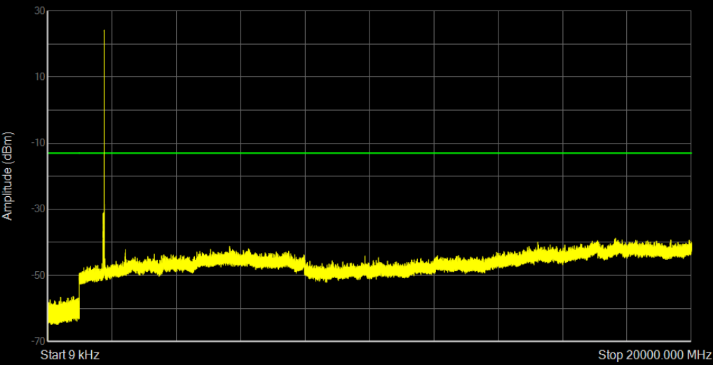
Band66 QPSK BW=1.4MHz Channel=132665 RB Size=6 Position=#0
