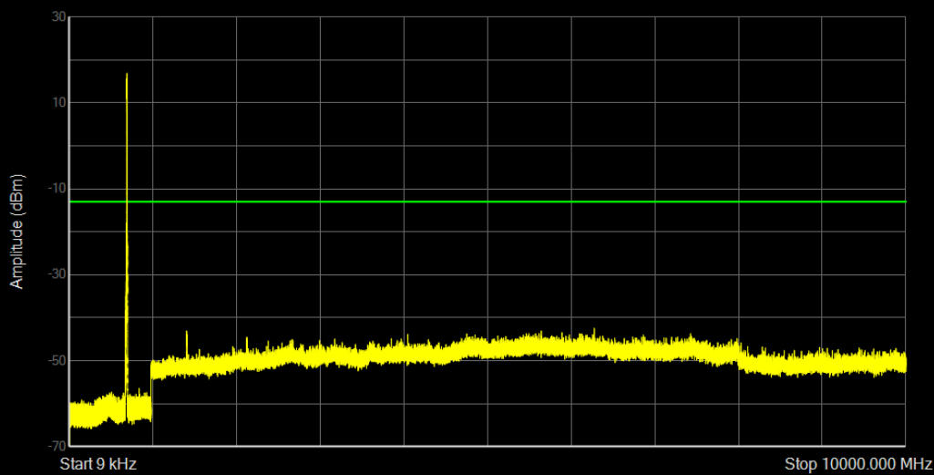
Band12 QPSK BW=5MHz Channel=23155 RB Size=25 Position=#0
