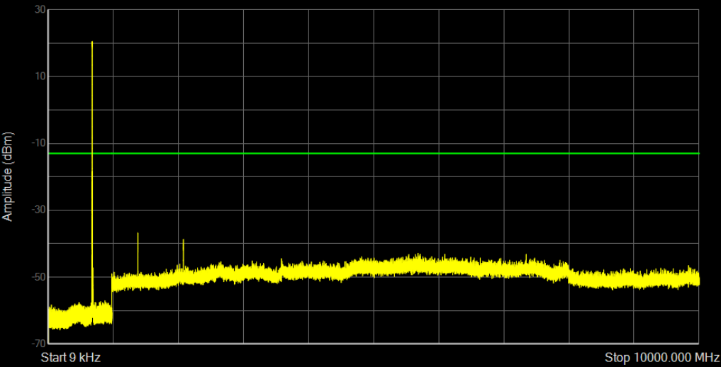
Band12 QPSK BW=1.4MHz Channel=23017 RB Size=6 Position=#0
