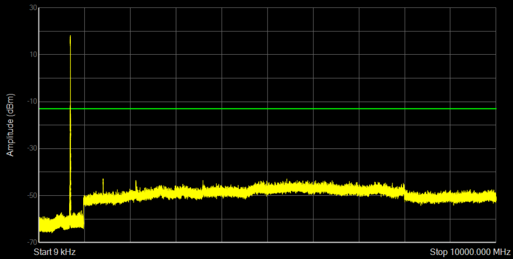
Band12 QPSK BW=3MHz Channel=23165 RB Size=15 Position=#0
