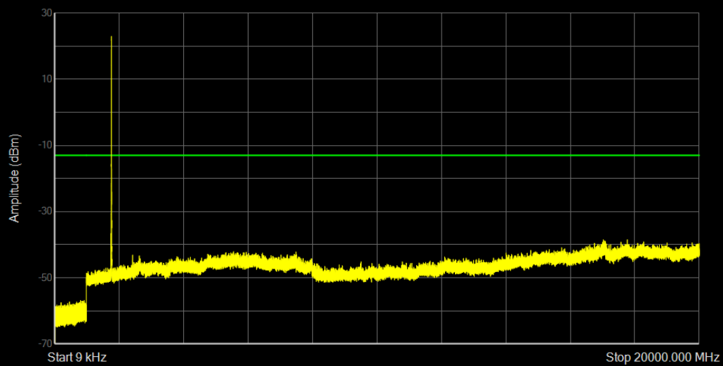
Band66 QAM16 BW=3MHz Channel=132657 RB Size=15 Position=#0
