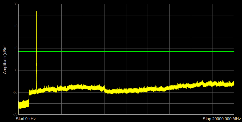
Band66 QPSK BW=3MHz Channel=131987 RB Size=15 Position=#0
