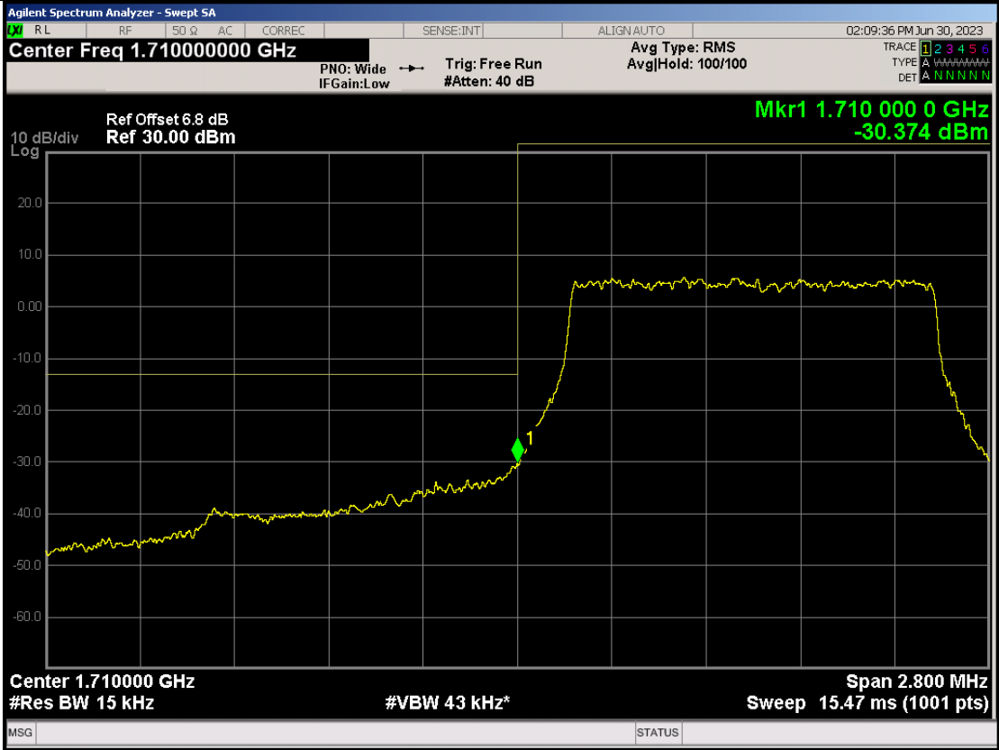
Band66 QPSK BW=1.4MHz Channel=131979 RB Size=6 Position=#0
