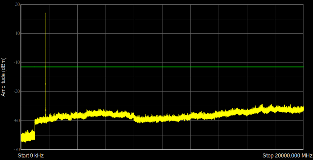
Band66 QAM16 BW=1.4MHz Channel=132665 RB Size=6 Position=#0
