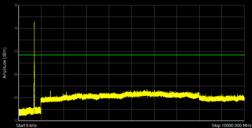
Band12 QAM16 BW=5MHz Channel=23155 RB Size=25 Position=#0
