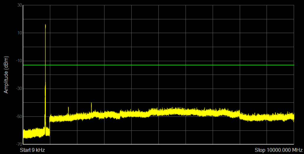
Band5 QPSK BW=3MHz Channel=20635 RB Size=15 Position=#0
