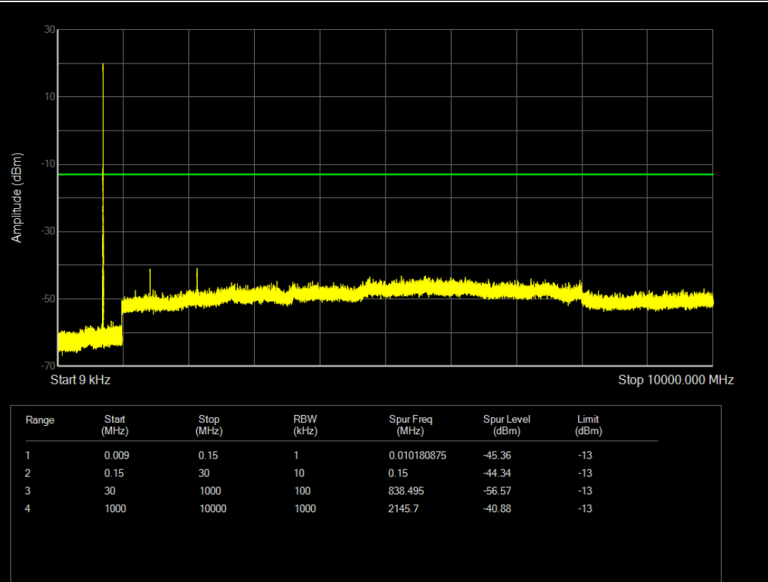
Band12 QAM16 BW=1.4MHz Channel=23173 RB Size=6 Position=#0
