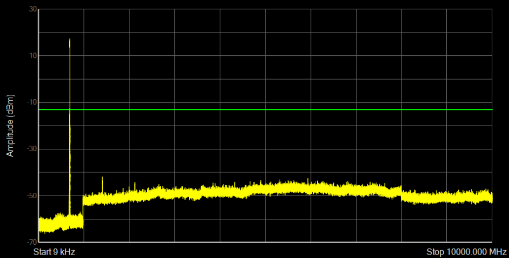
Band12 QAM16 BW=3MHz Channel=23165 RB Size=15 Position=#0
