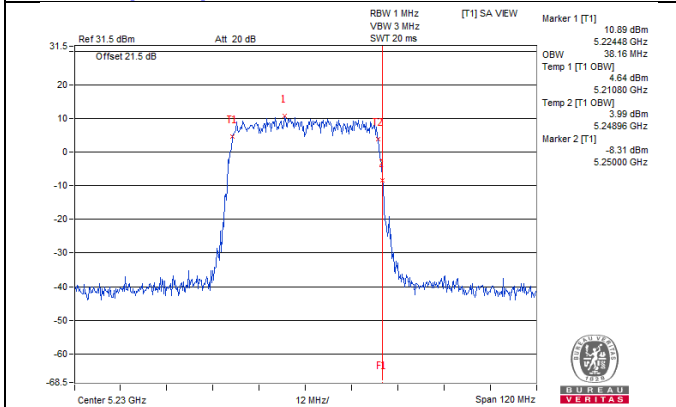
802.11ax (HE40) Chain 6 / CH46
