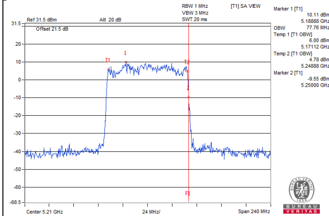
802.11ax (HE80+80) / Chain 2 : CH42
