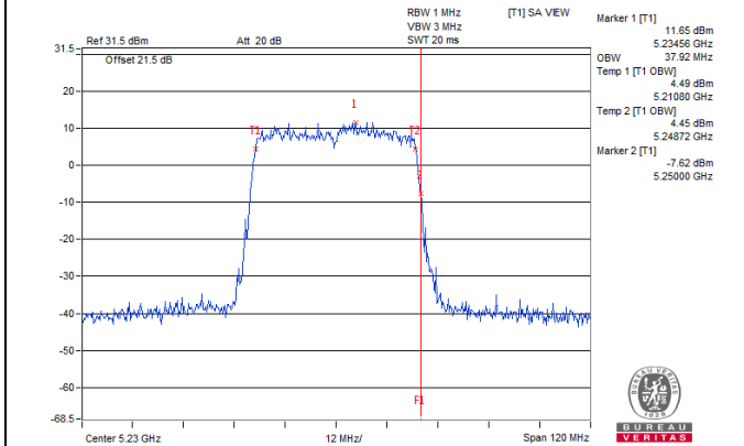
802.11ax (HE40) Chain 4 / CH46
