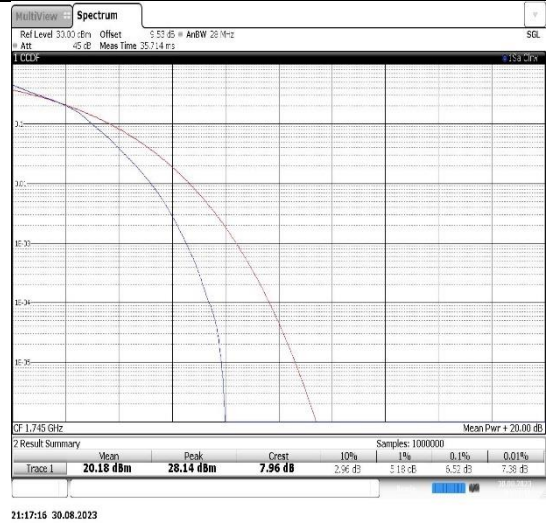
Band66-15MHz-16QAM-132322-75RB#0
