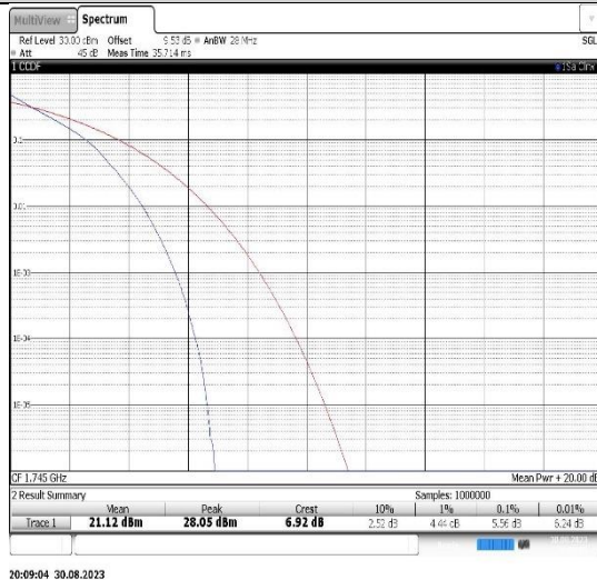
Band66-5MHz-QPSK-132322-1RB#0
