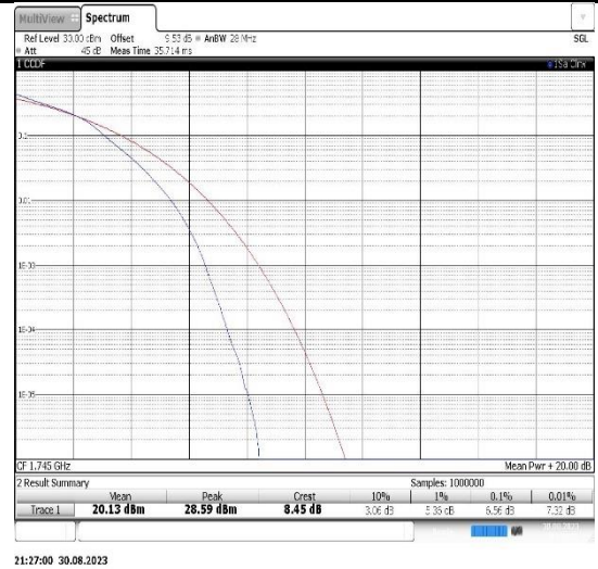
Band66-20MHz-16QAM-132322-100RB#0
