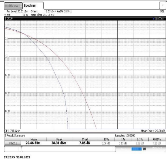
Band66-3MHz-16QAM-132322-15RB#0
