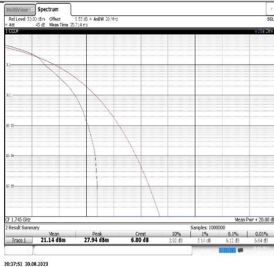
Band66-10MHz-QPSK-132322-50RB#0
