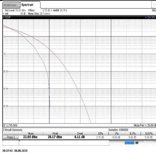
Band66-5MHz-16QAM-132322-1RB#0
