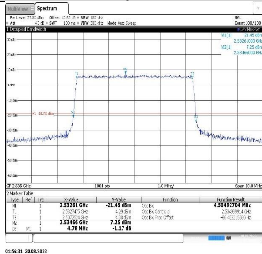
Band7-10MHz-16QAM-21100-50RB#0
