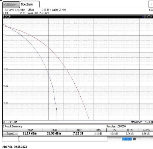
Band66-15MHz-QPSK-132322-75RB#0
