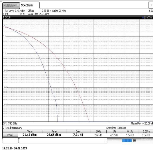
Band66-3MHz-QPSK-132322-15RB#0
