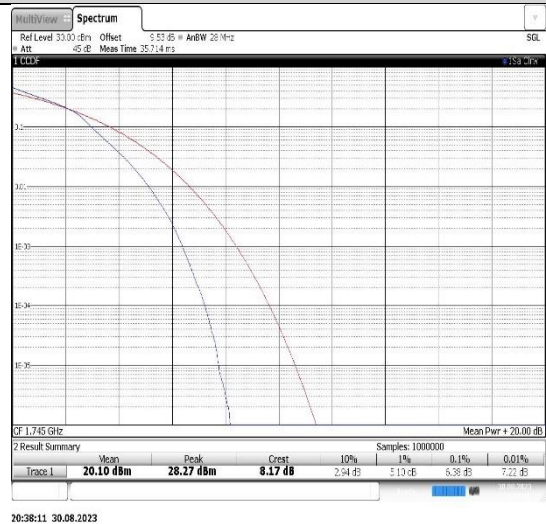
Band66-10MHz-16QAM-132322-50RB#0
