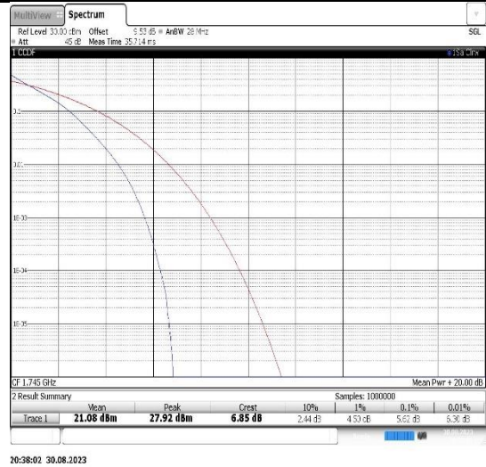
Band66-5MHz-16QAM-132322-25RB#0
