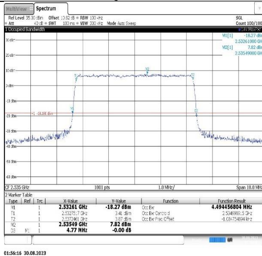
Band7-10MHz-QPSK-21100-50RB#0
