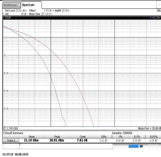
Band66-20MHz-QPSK-132322-100RB#0
