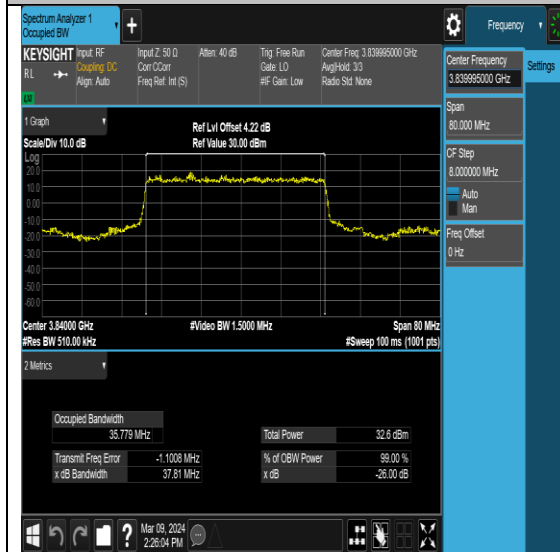
NTNV-N77-3700-3980-PC2-30-40-M-DFT- PI2BPSK-Outer_Full-Ant1-PASS
