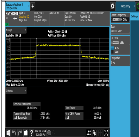
NTNV-N77-3700-3980-PC2-30-40-M-DFT- 256QAM-Outer_Full-Ant1-PASS
