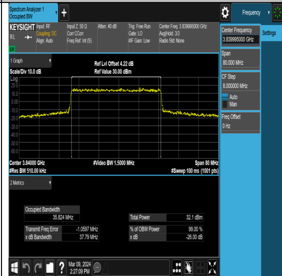
NTNV-N77-3700-3980-PC2-30-40-M-DFT-QPSK- Outer_Full-Ant1-PASS
