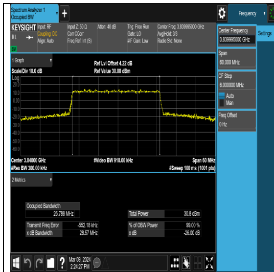
NTNV-N77-3700-3980-PC2-30-30-M-DFT- 64QAM-Outer_Full-Ant1-PASS
