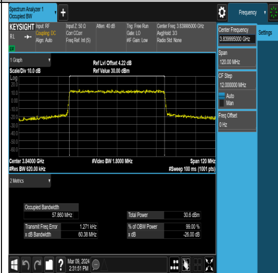
NTNV-N77-3700-3980-PC2-30-60-M-DFT-256QAM-Outer_Full-Ant1-PASS
