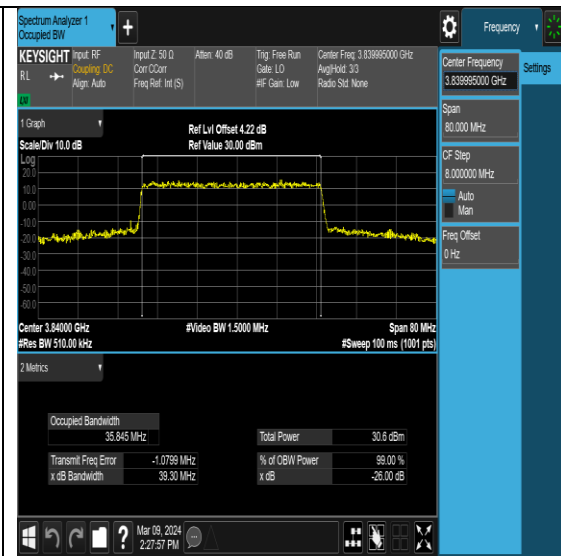
NTNV-N77-3700-3980-PC2-30-40-M-DFT- 64QAM-Outer_Full-Ant1-PASS
