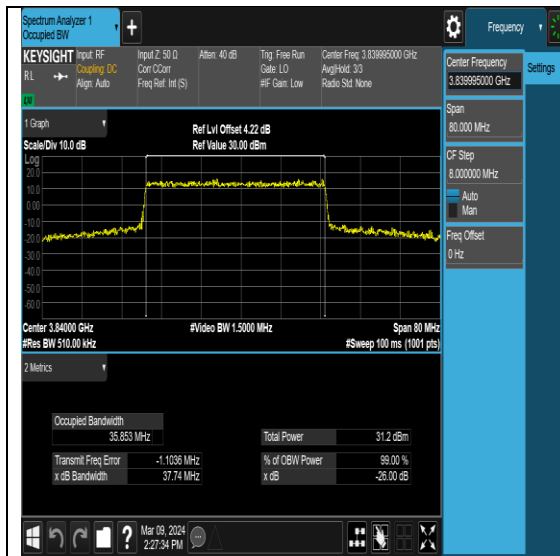
NTNV-N77-3700-3980-PC2-30-40-M-DFT- 16QAM-Outer_Full-Ant1-PASS
