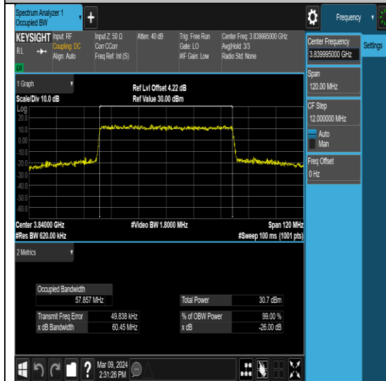
NTNV-N77-3700-3980-PC2-30-60-M-DFT-64QAM-Outer_Full-Ant1-PASS
