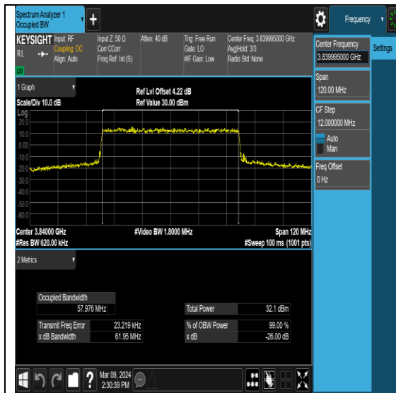
NTNV-N77-3700-3980-PC2-30-60-M-DFT-QPSK-Outer_Full-Ant1-PASS
