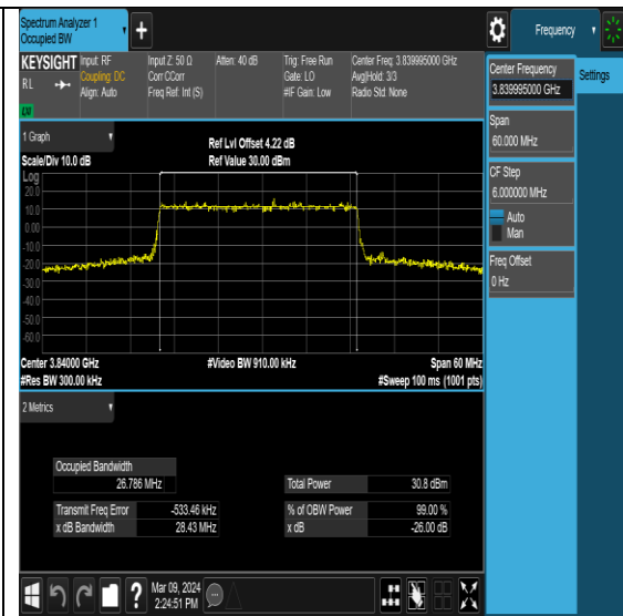
NTNV-N77-3700-3980-PC2-30-30-M-DFT- 256QAM-Outer_Full-Ant1-PASS
