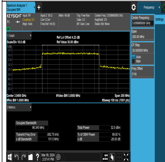
NTNV-N77-3700-3980-PC2-30-100-M-DFT- QPSK-Outer_Full-Ant1-PASS
