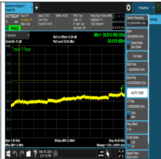
NTNV-N77-3700-3980-PC2-30-60-M-DFT-QPSK- Edge_1RB_Left-Ant1-PASS
