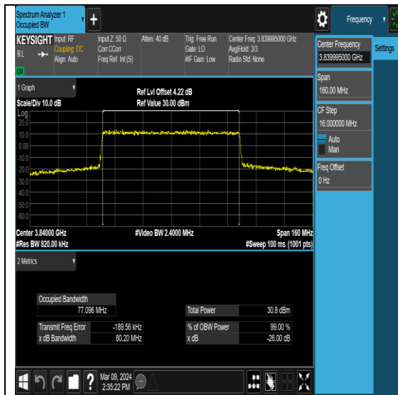
NTNV-N77-3700-3980-PC2-30-80-M-DFT- 256QAM-Outer_Full-Ant1-PASS
