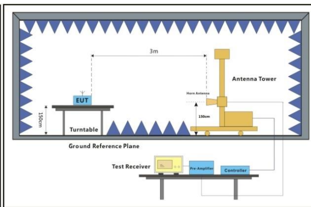
Above 1GHz
